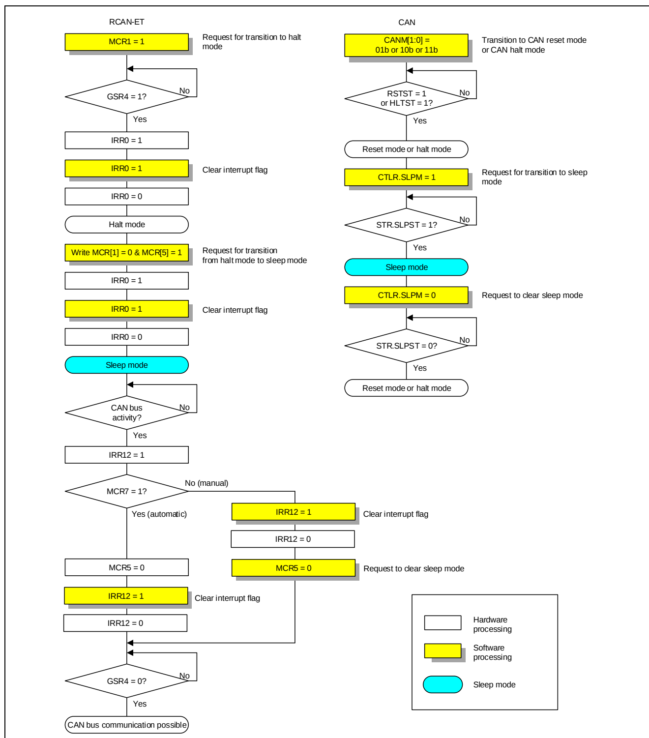
Figure 4.1 Sleep Mode Setting Procedure on SH7137 (RCAN-ET) and RX65N (CAN)
