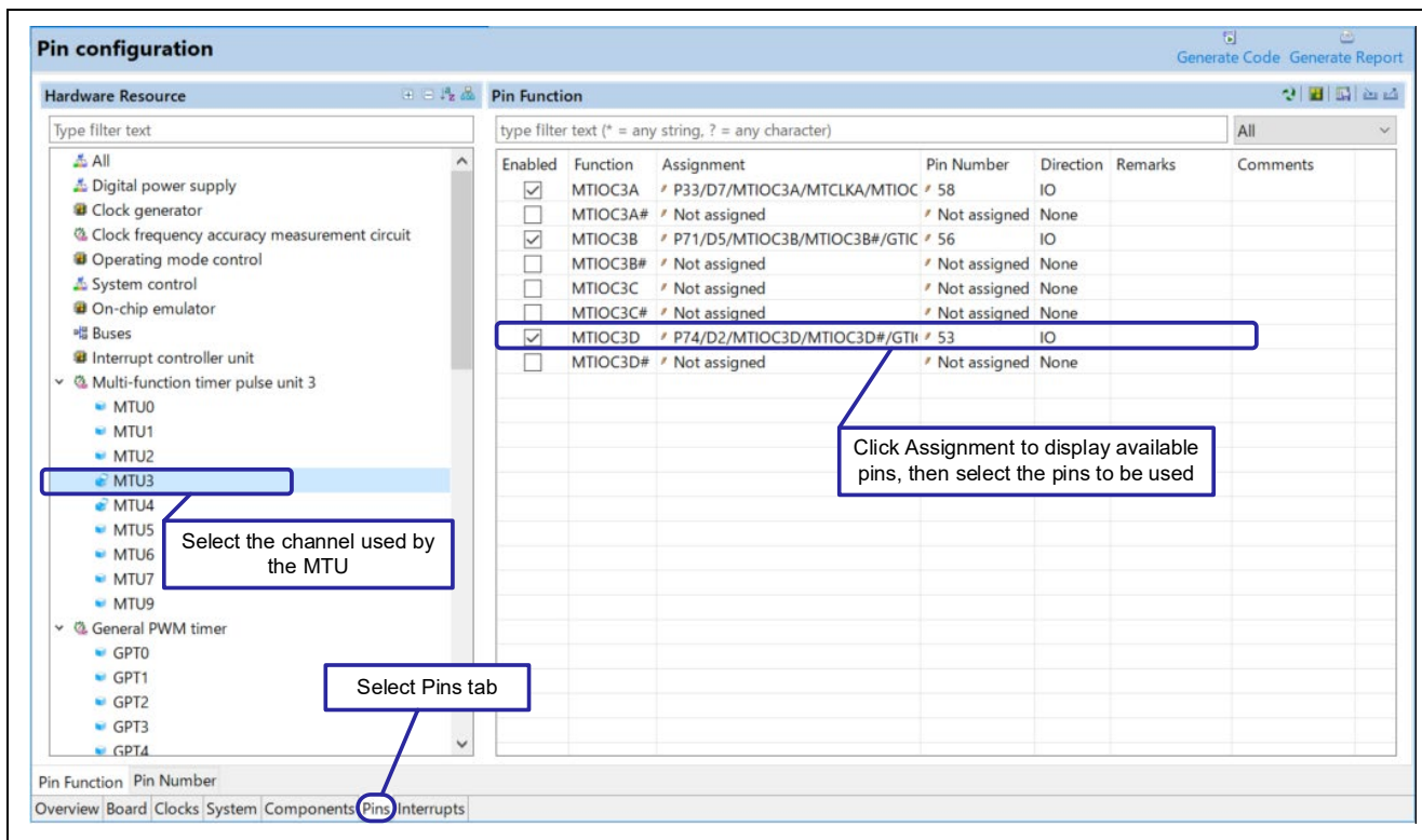
Figure 3.3 Pin Settings
