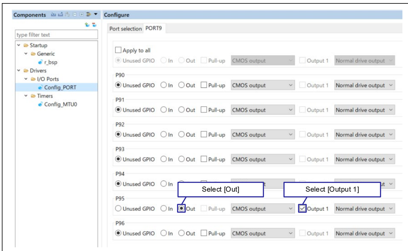
Figure 3.9 P95 Settings (2/2)
