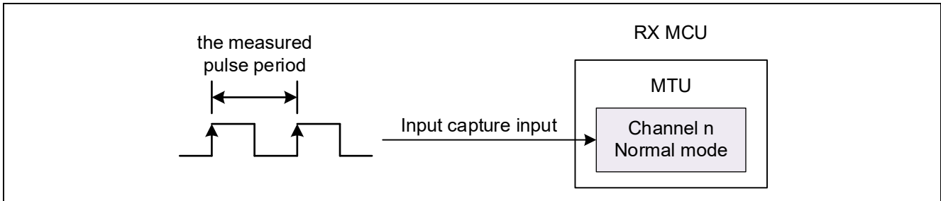
Figure 1.1 Measuring a Pulse Period
