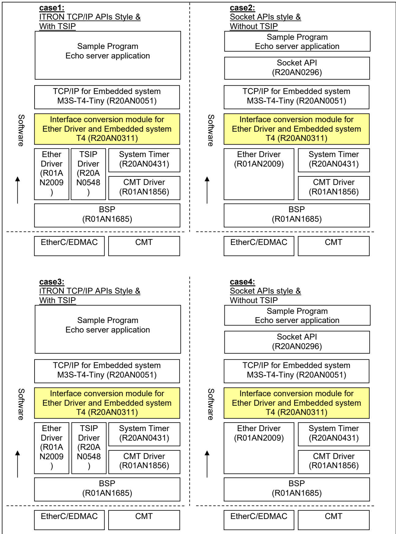
Figure 1 Software stack about T4 Driver FIT Modules
