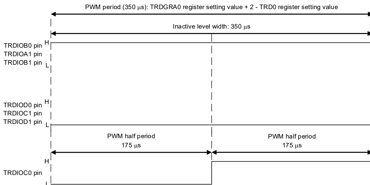
Figure 4.4 PWM Waveform 4
