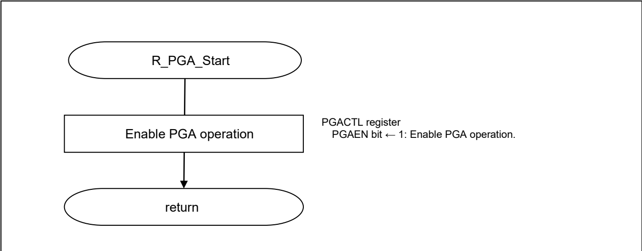
Figure 4.26 PGA Startup
