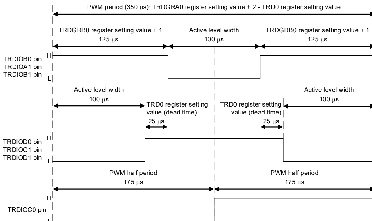
Figure 4.2 PWM Waveform 2
