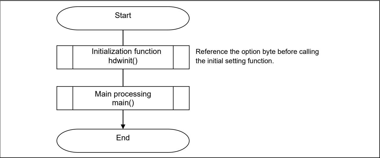
Figure 4.12 Entire Flow
