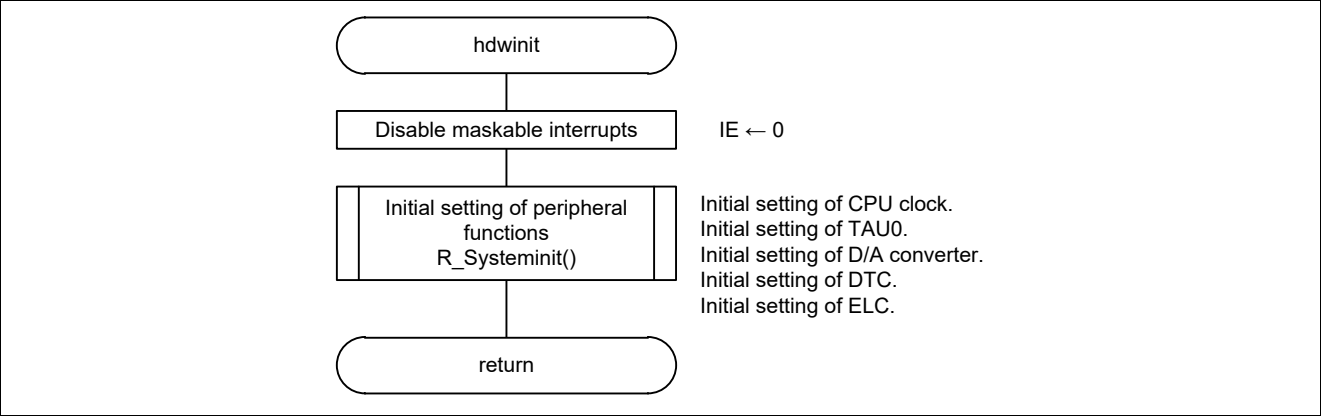
Figure 4.3 Initial Setting
