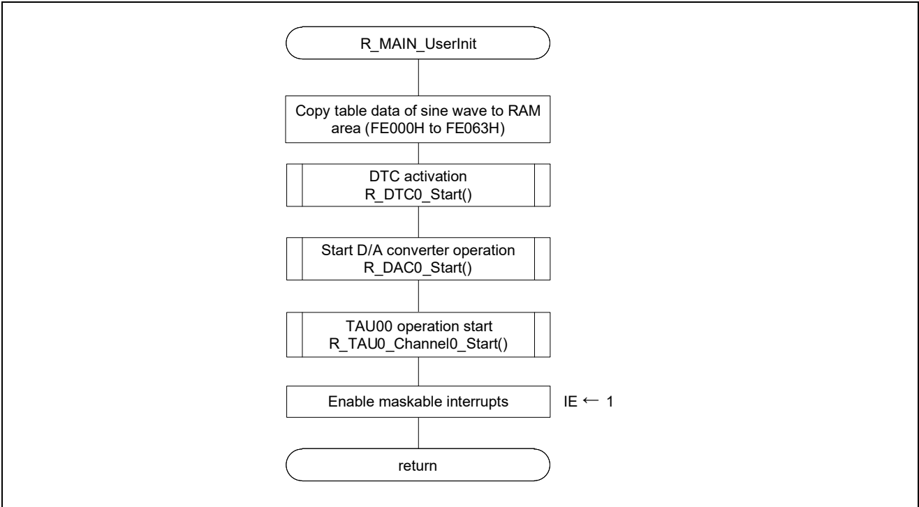
Figure 4.11 Main Initialization
