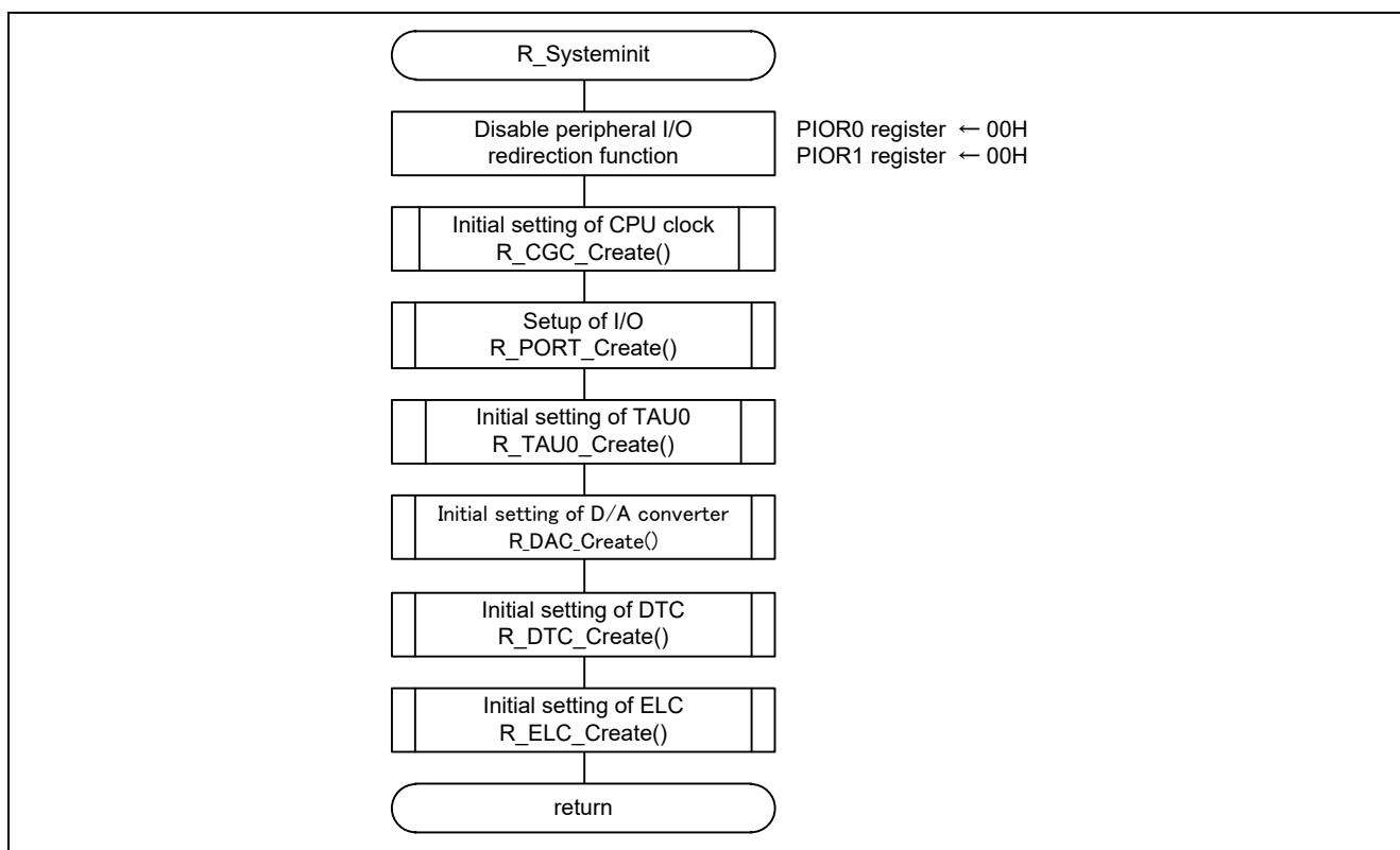
Figure 4.4 Initial Setting of Peripheral Functions
