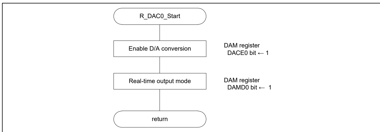
Figure 4.13 DAC0 Conversion Start Setting
