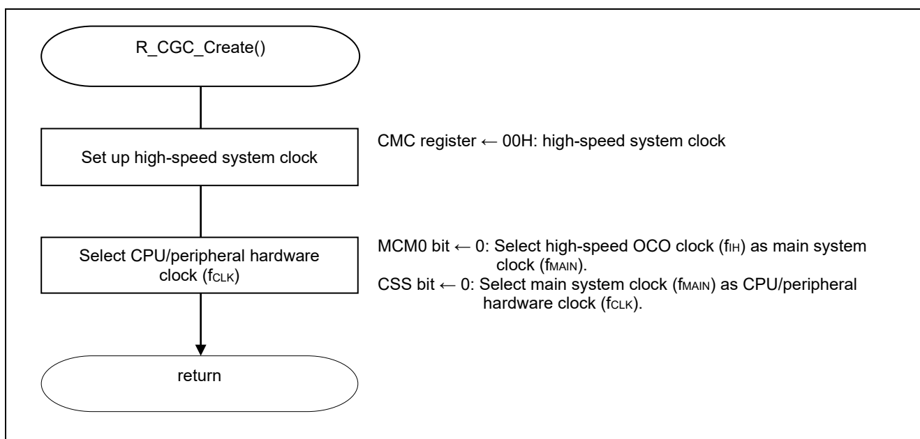
Figure 4.5 Initial Setting of the CPU Clock
