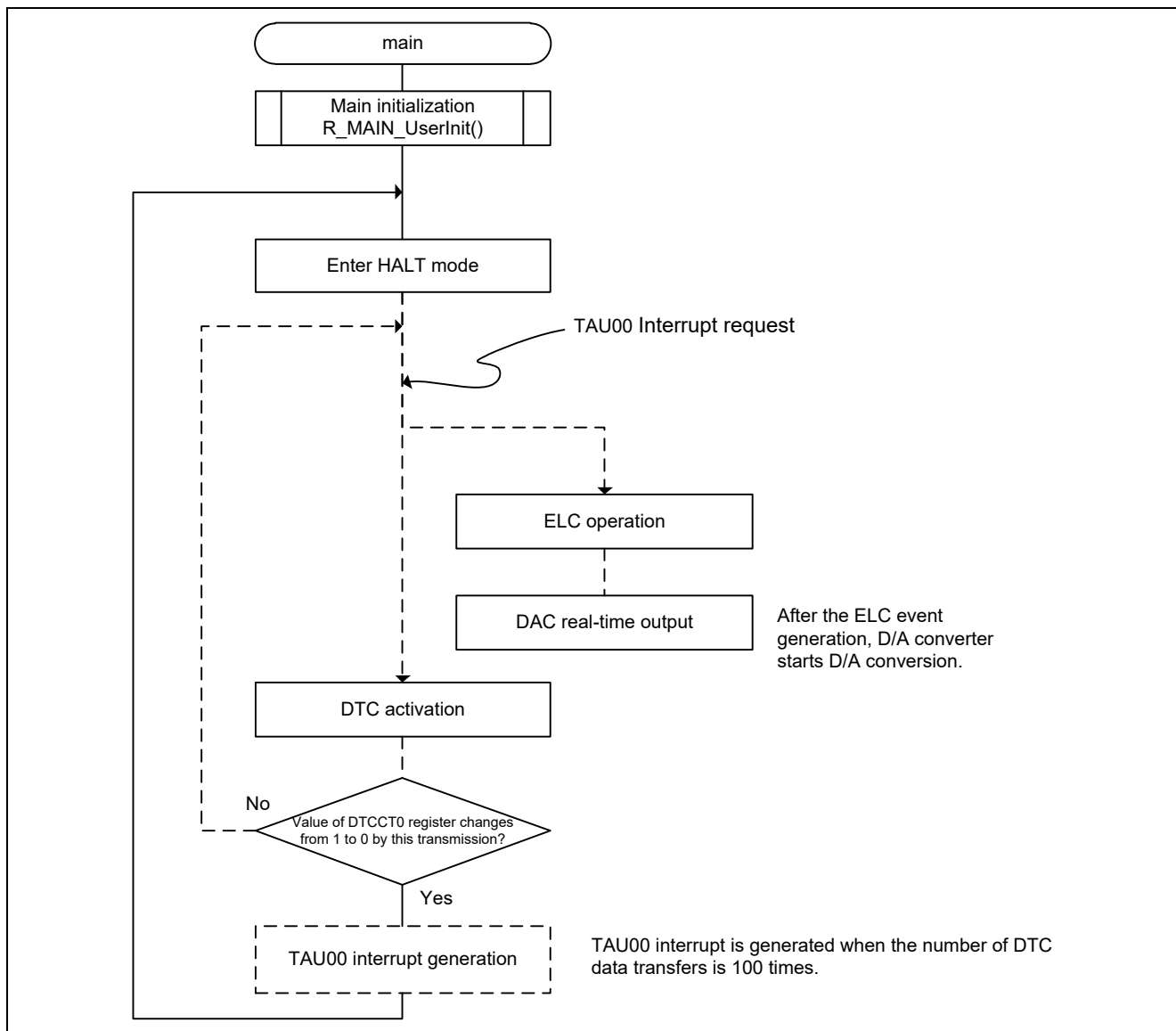
Figure 4.10 Main Processing
