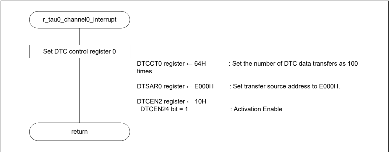
Figure 4.15 TAU00 Interrupt
