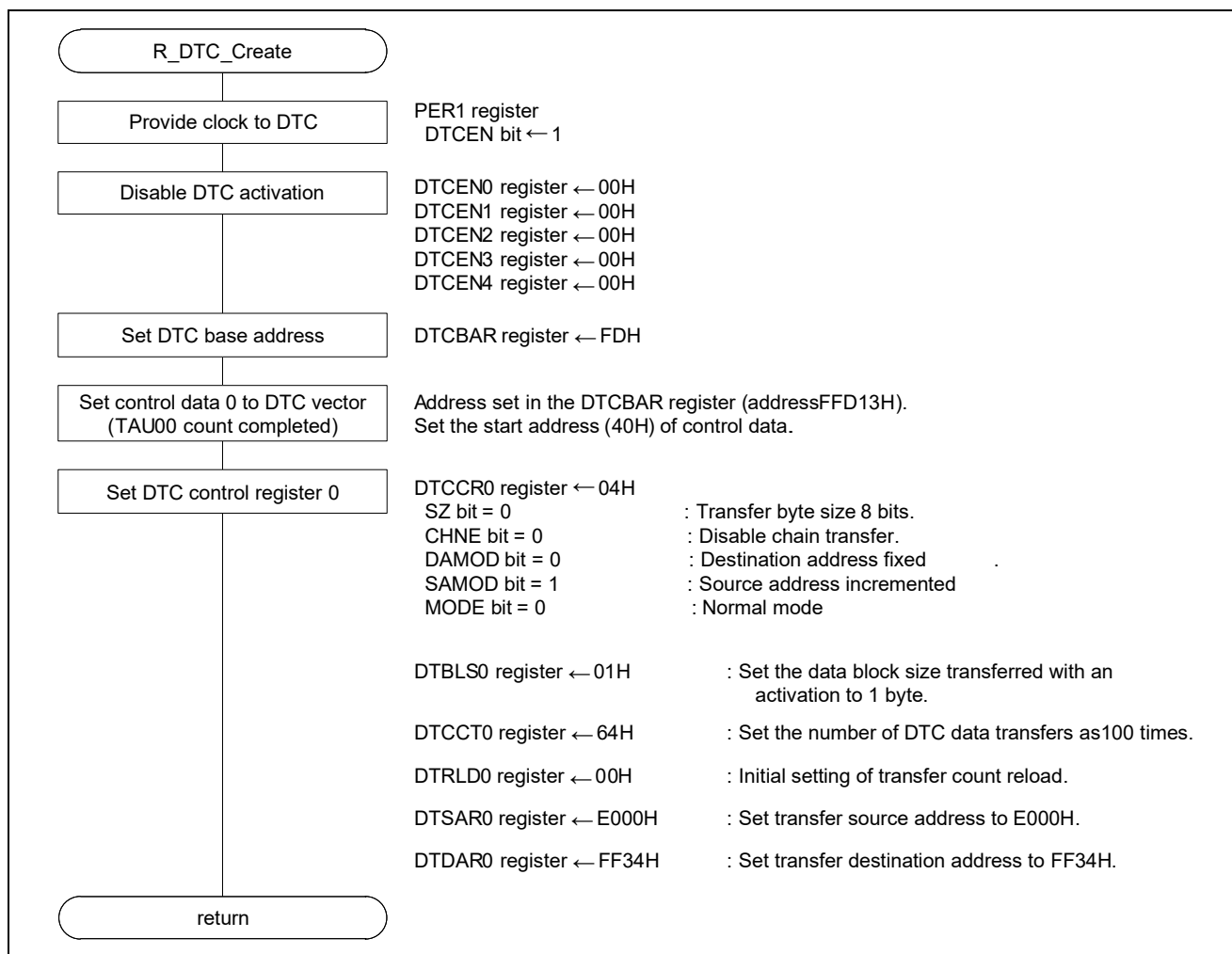
Figure 4.8 Initial Setting of the DTC
