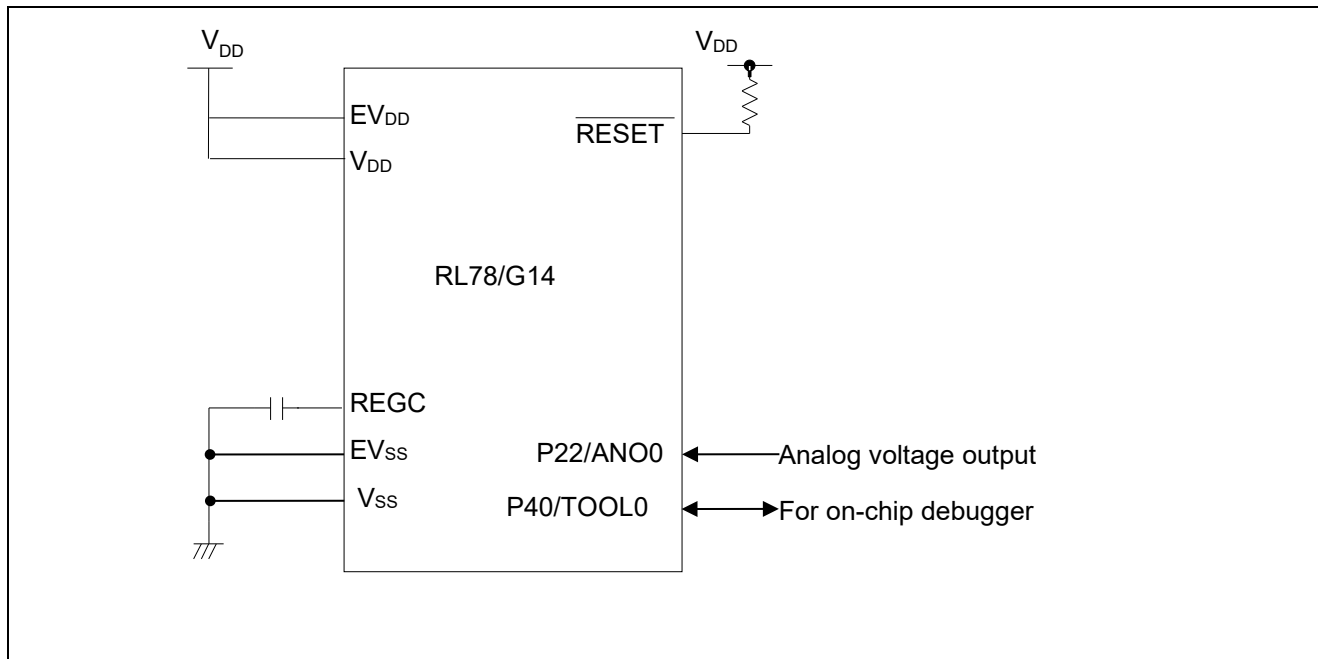
Figure 3.1 Hardware Configuration
