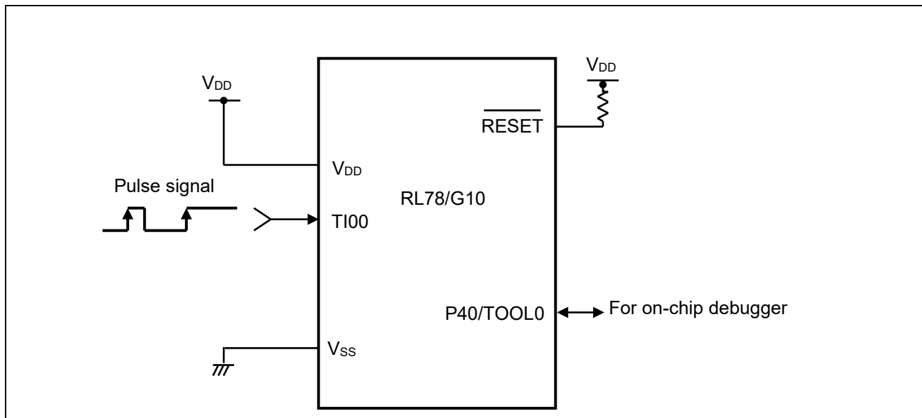
Figure 4.1 Hardware Configuration
