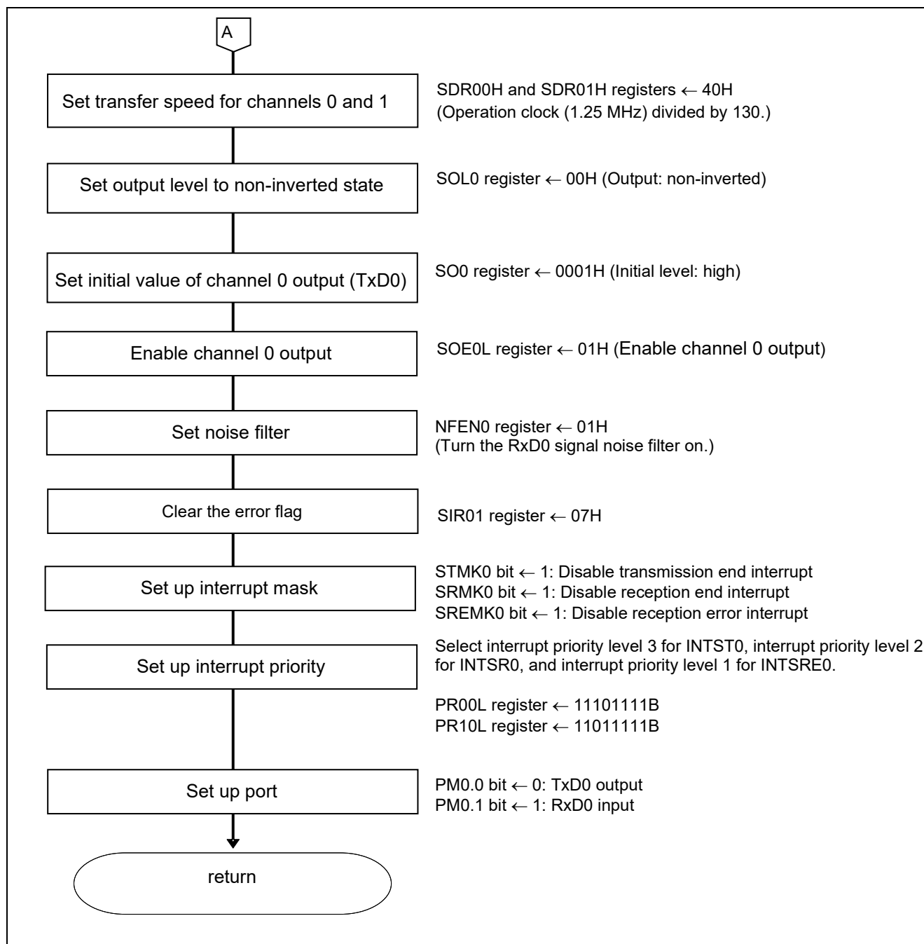
Figure 5.5 SAU Setup (2/2)
