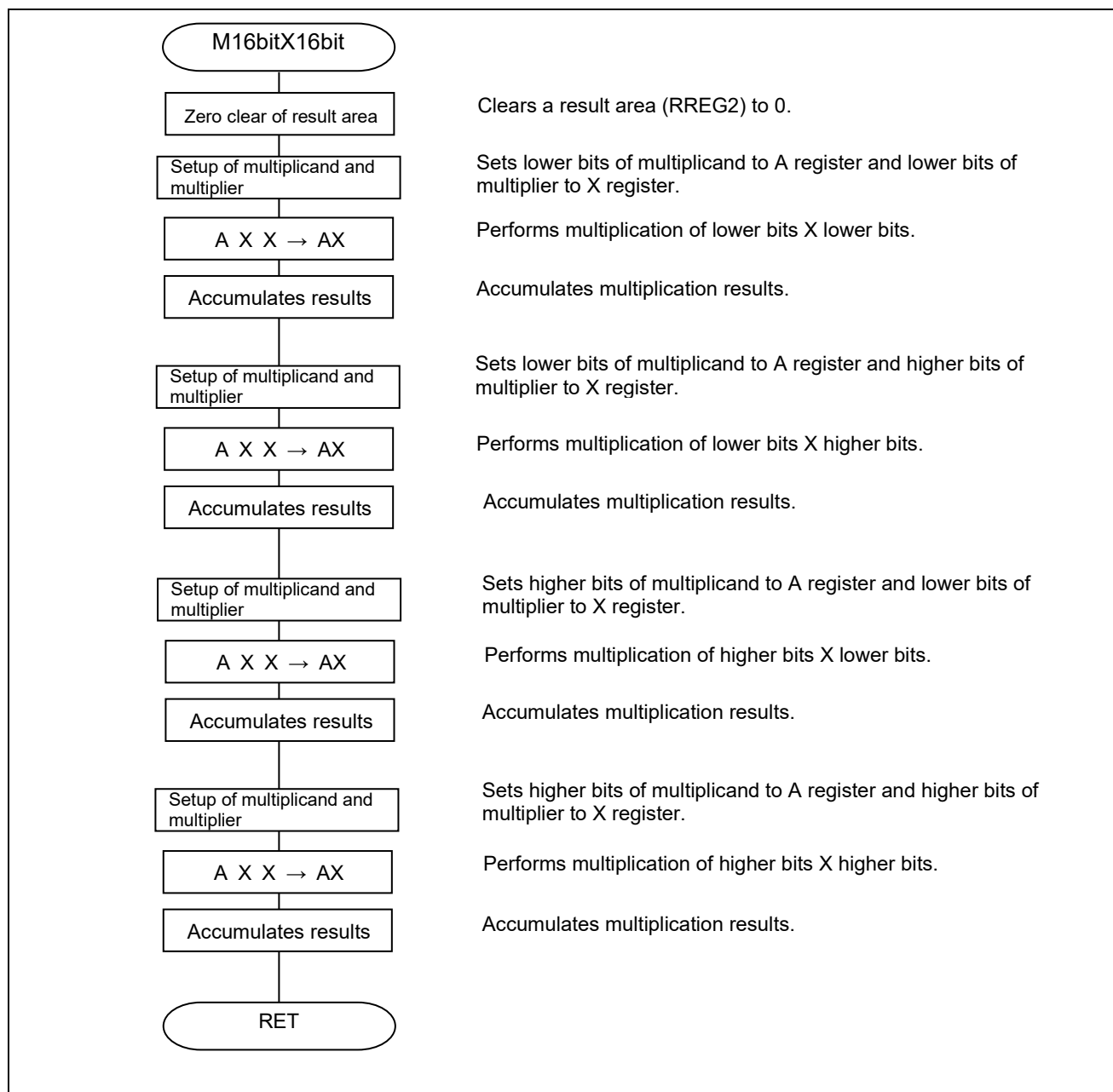
Figure 3.9 Multiplication Processing of 16 Bits Data
