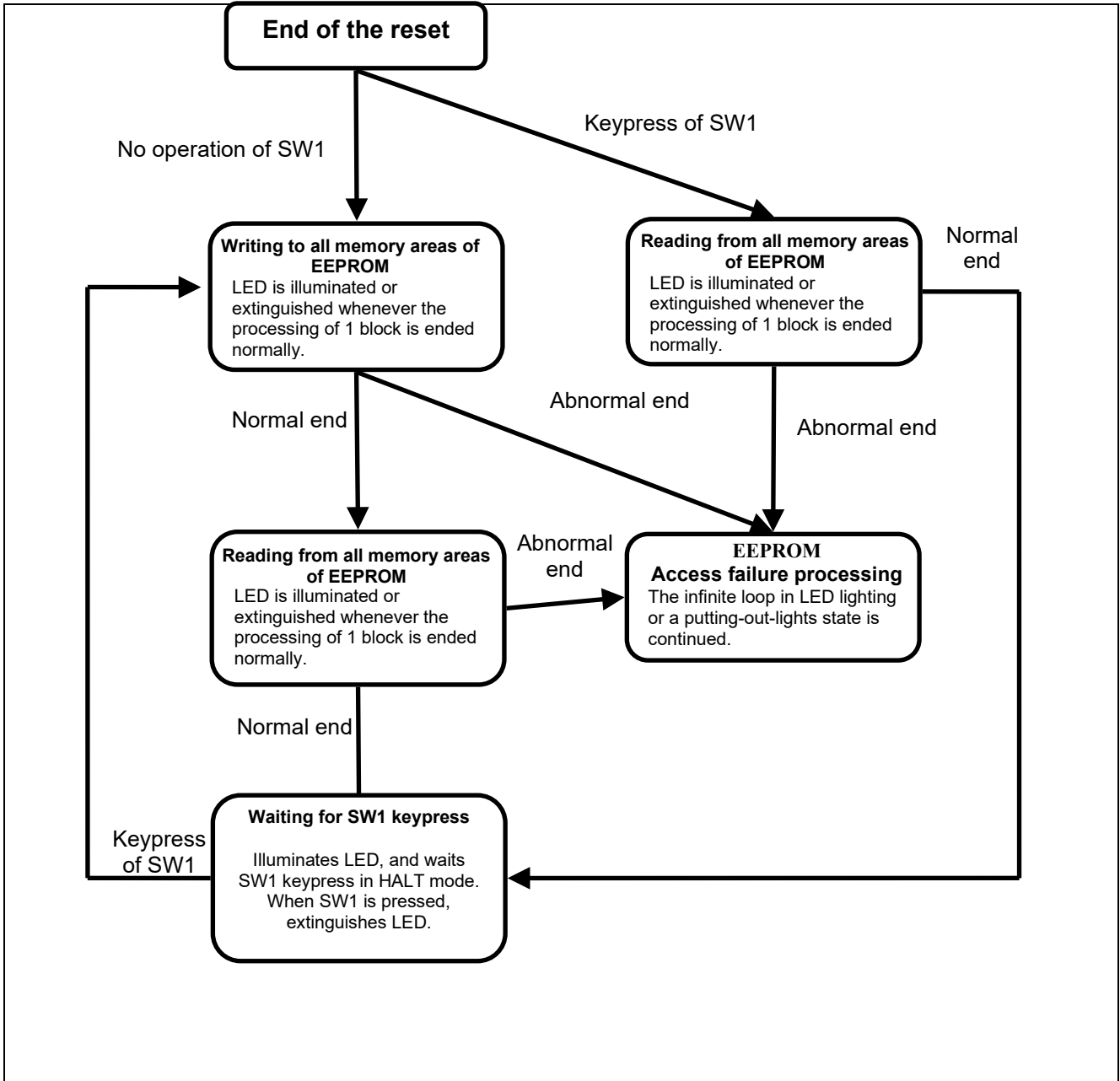
Figure 1.1 Operation Outline
