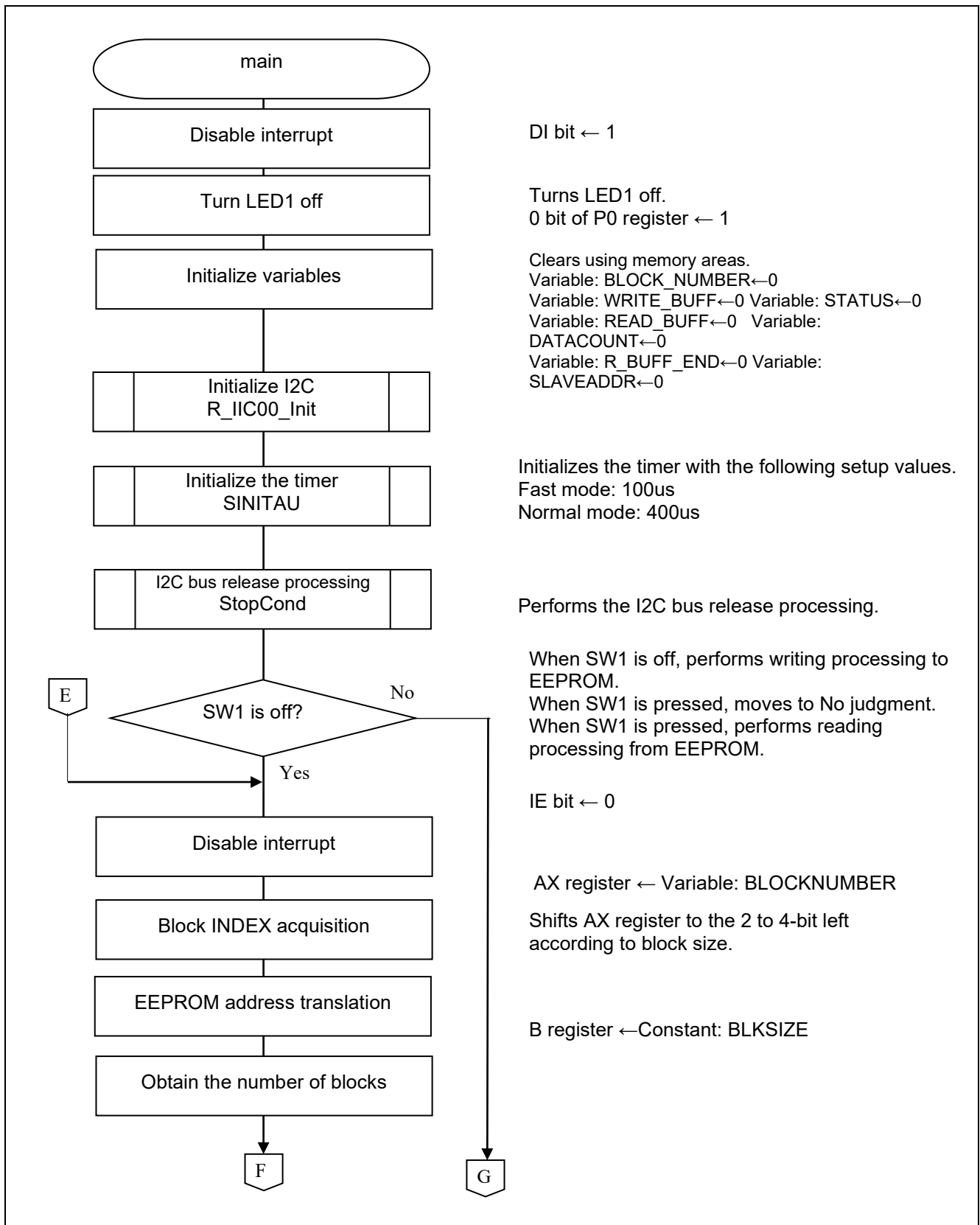
Figure 5.10 Main Processing (1/4)
