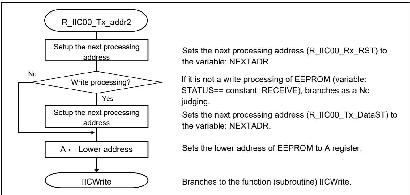
Figure 5.17 EEPROM Lower Address Transmitting (R_IIC00_Tx_addr2)
