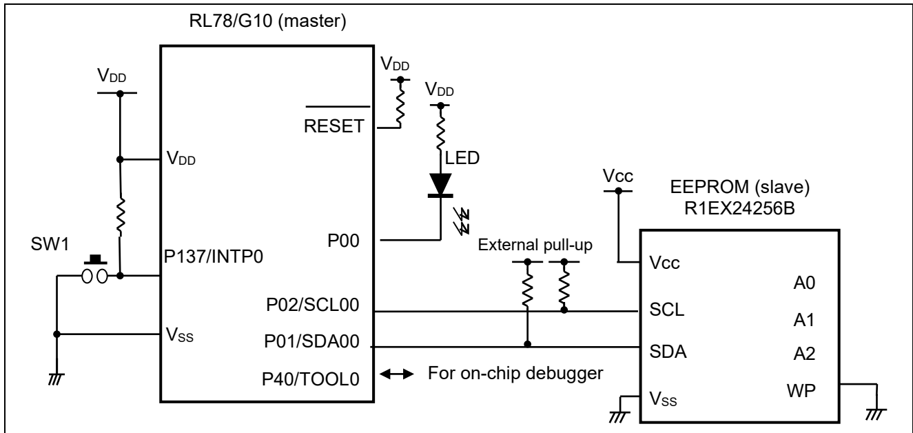
Figure 4.1 Hardware Configuration
