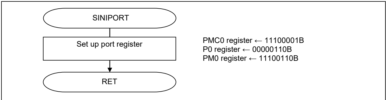
Figure 5.7 I/O Port Setup Function
