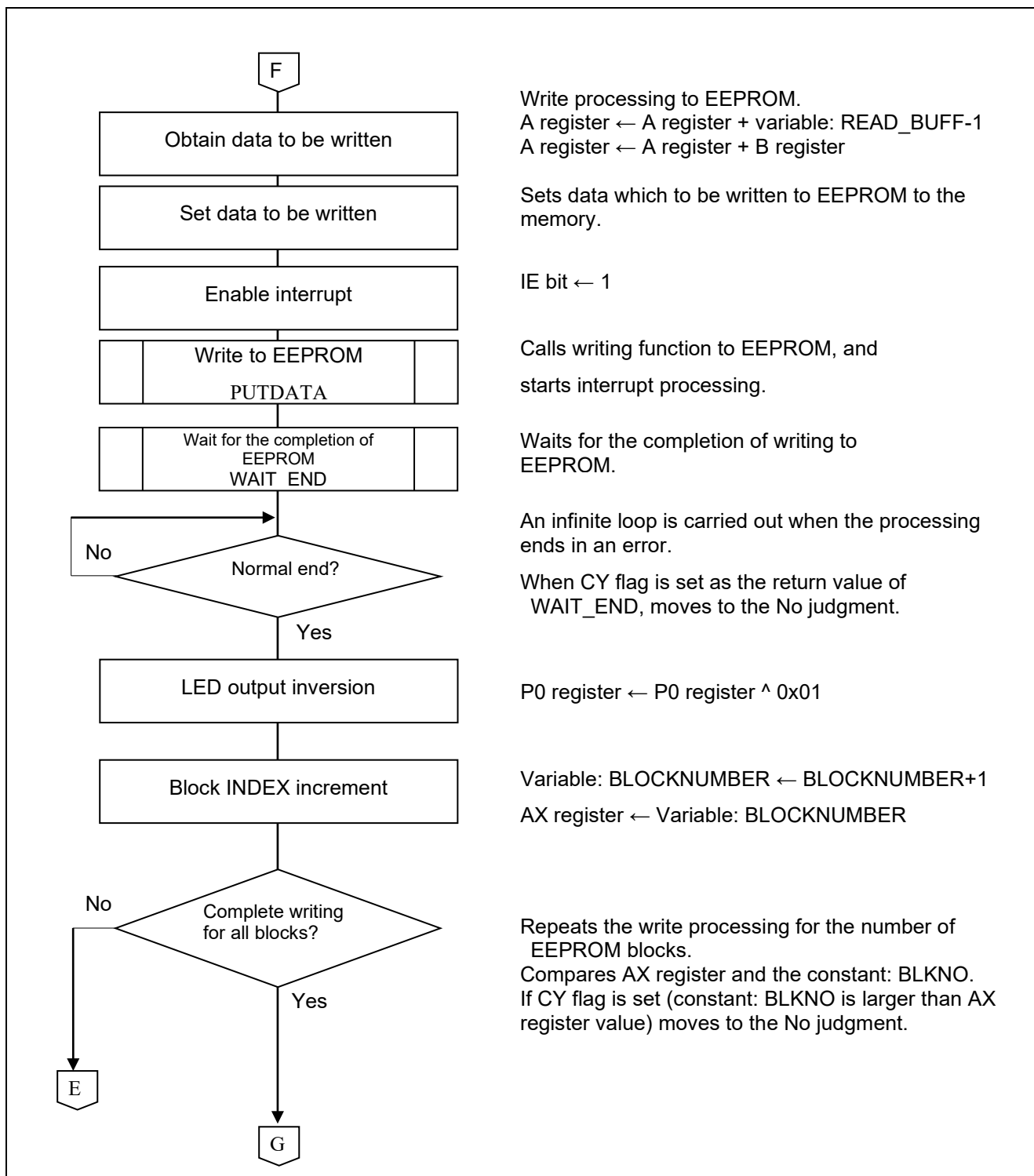
Figure 5.11 Main Processing (2/4)
