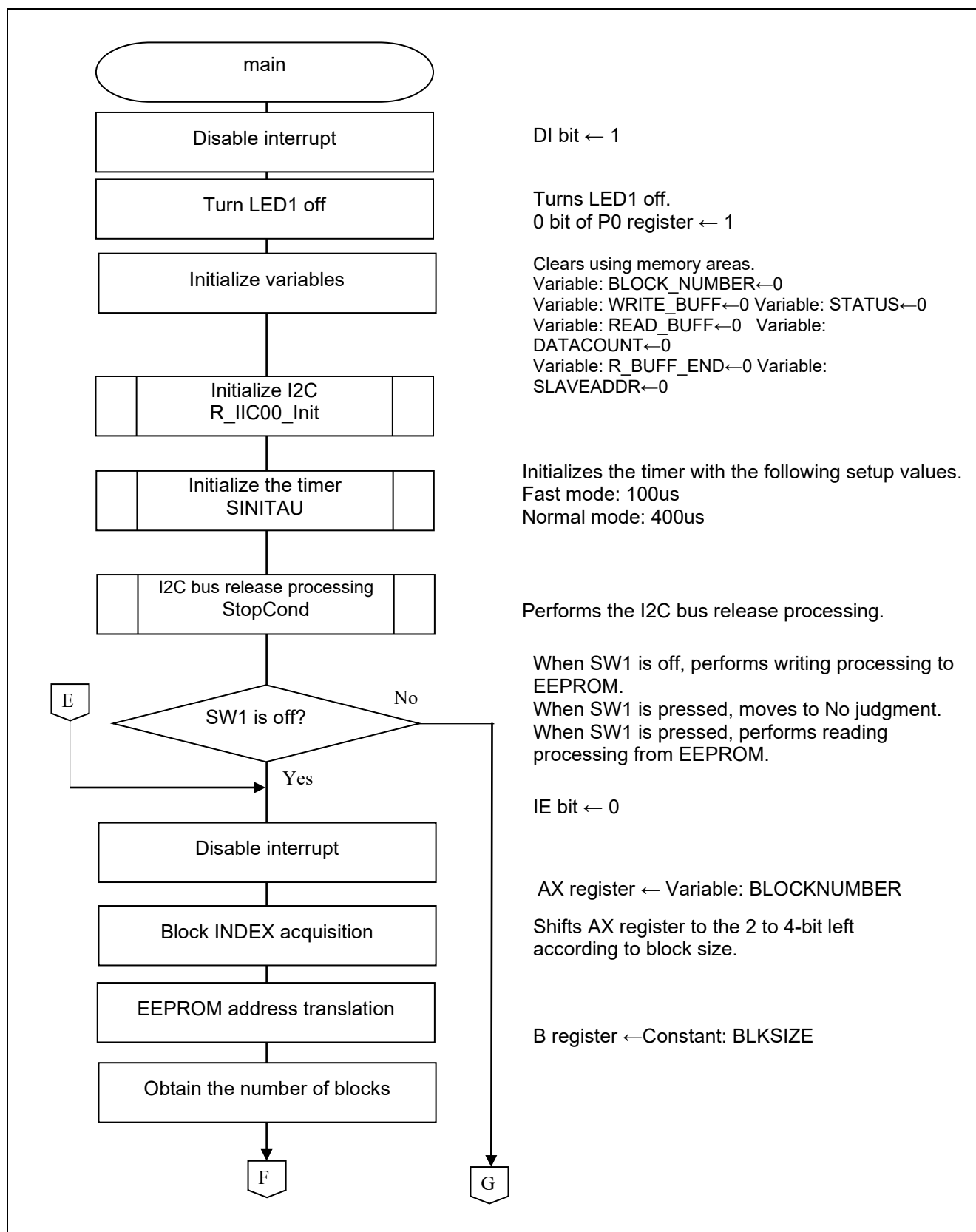
Figure 5.10 Main Processing (1/4)
