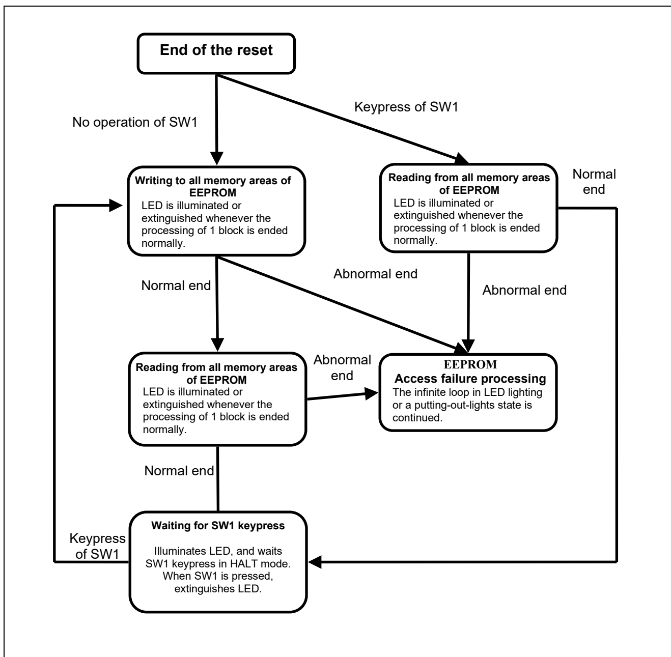
Figure 1.1 Operation Outline
