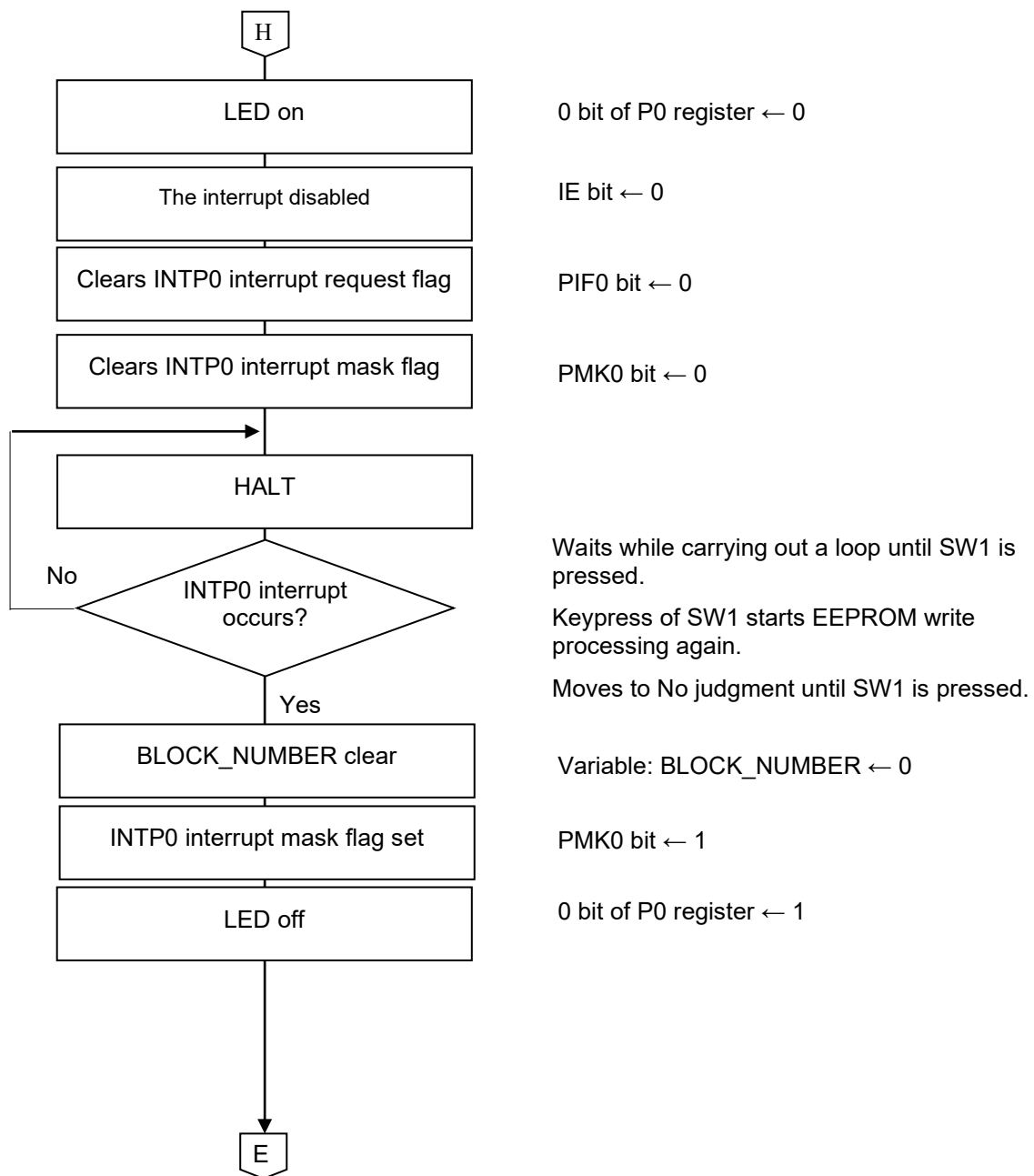
Figure 5.13 Main Processing (4/4)
