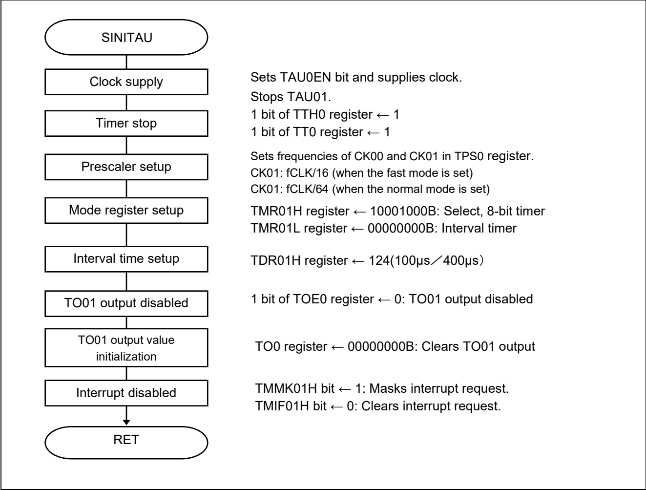
Figure 5.33 Timer Initialization
