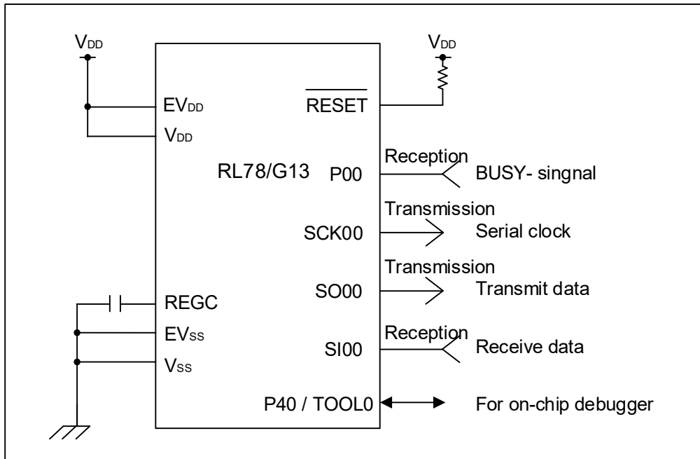
Figure 3-1 Hardware Configuration Example (Porting Example 1)
