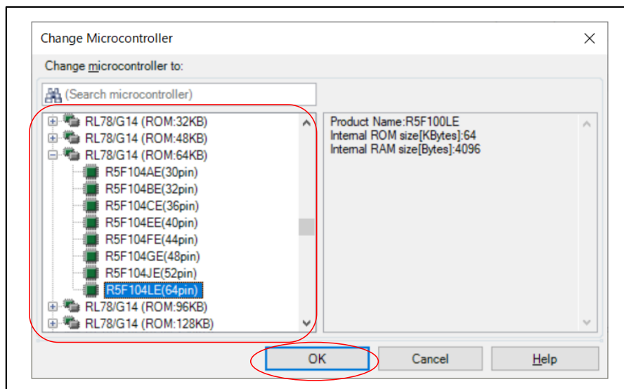
Figure 2-3 [Change Microcontroller]
