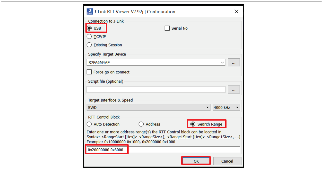
Figure 68. SEGGER RTT Viewer Connection Setup when MCU Running in Standalone Mode
