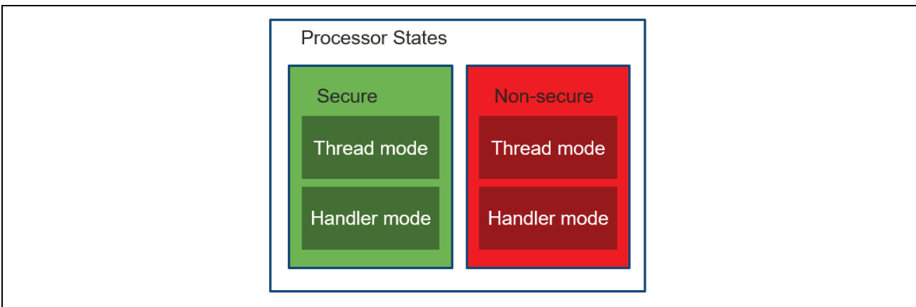
Figure 1. Processor States
