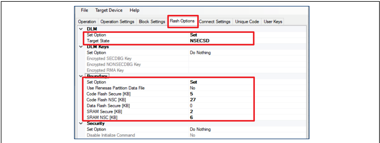
Figure 92. Setup for the IDAU Region
