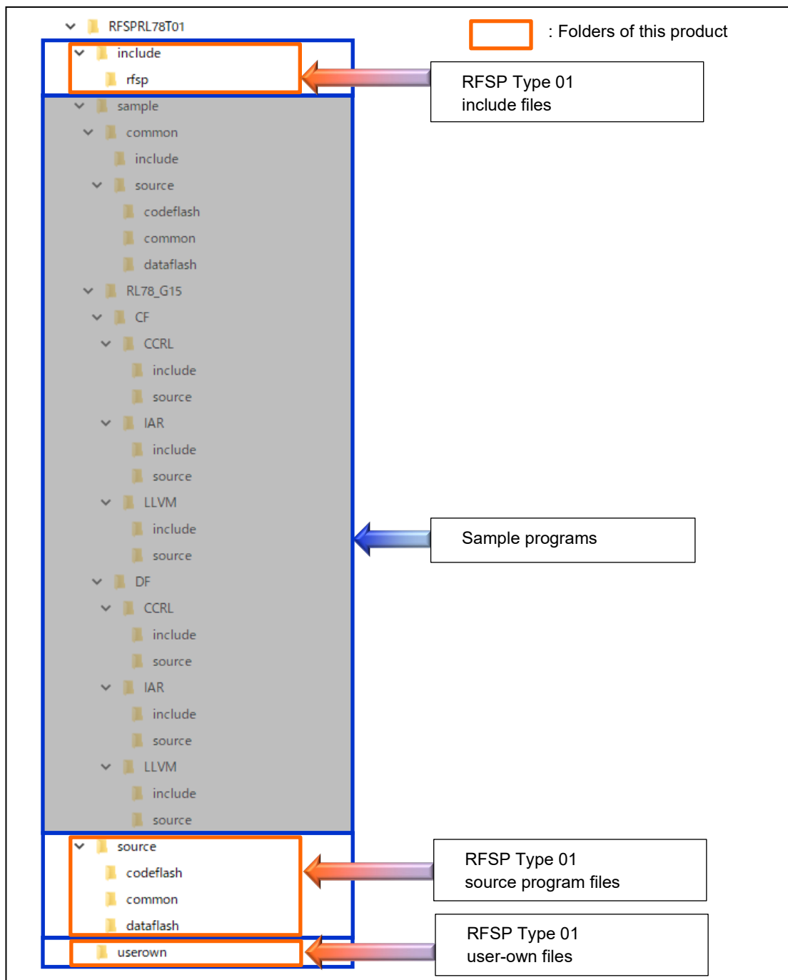
Figure 2-1 Folder Structure of RFSP Type 01
