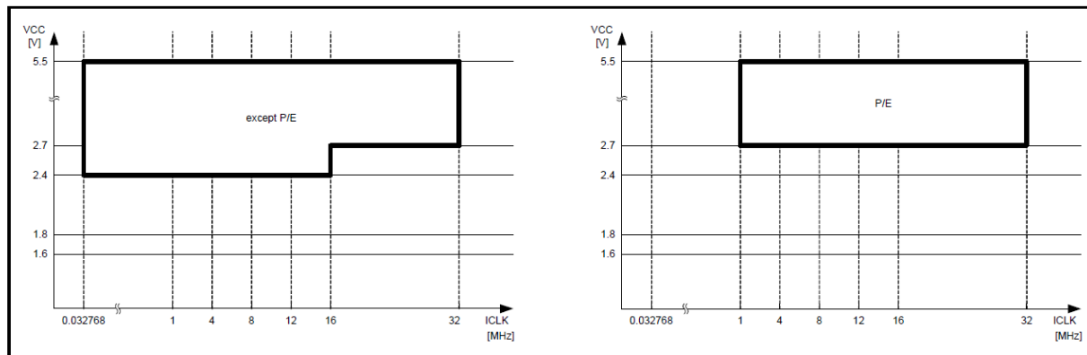
Figure 1. System clock range for High-speed mode
