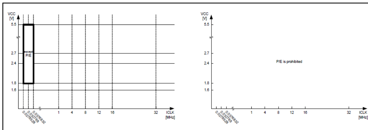
Figure 5. System clock range for the Subosc-speed mode
