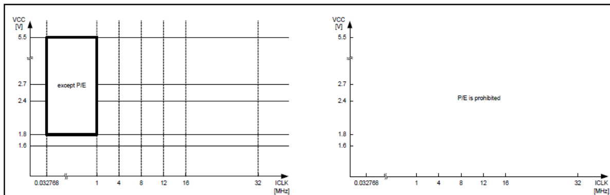
Figure 4. System clock range for the Low-speed mode
