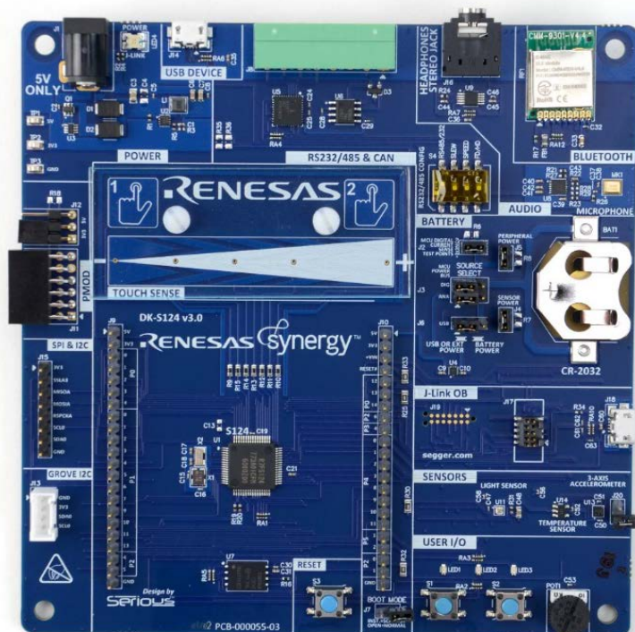
Figure 7. DK-S124 v3.0 Synergy MCU board
