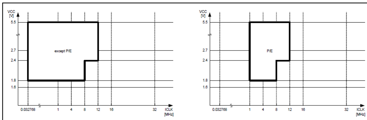
Figure 2. System clock range for Middle-speed mode
