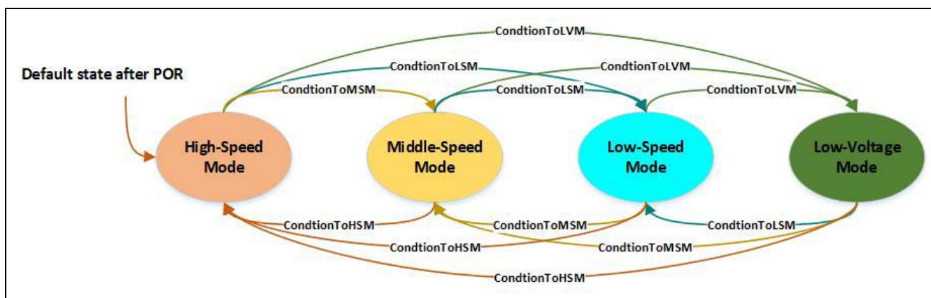
Figure 9. FSM1 state transition diagram
