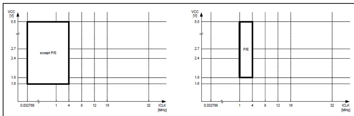
Figure 3. System clock range for low-voltage mode
