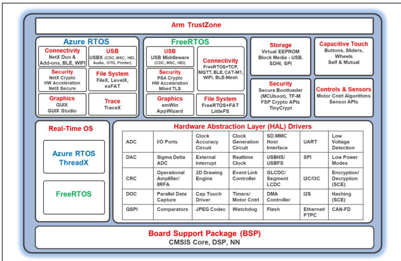
Figure 5. Flexible Software Package (FSP)
