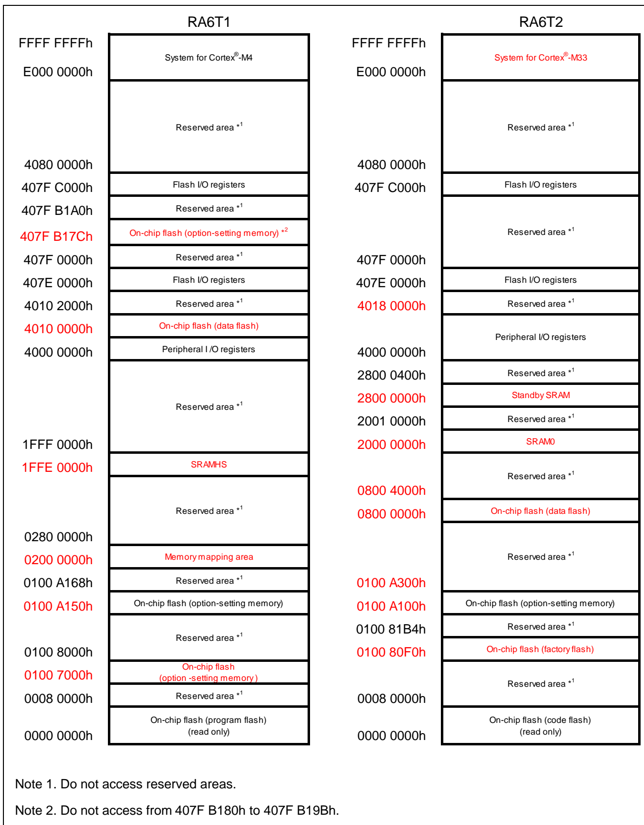
Figure 1. Comparison of Memory Maps
