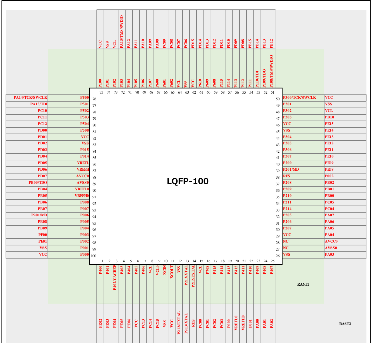
Figure 3. Comparison of Pin Assignment for the 100-pin Package
