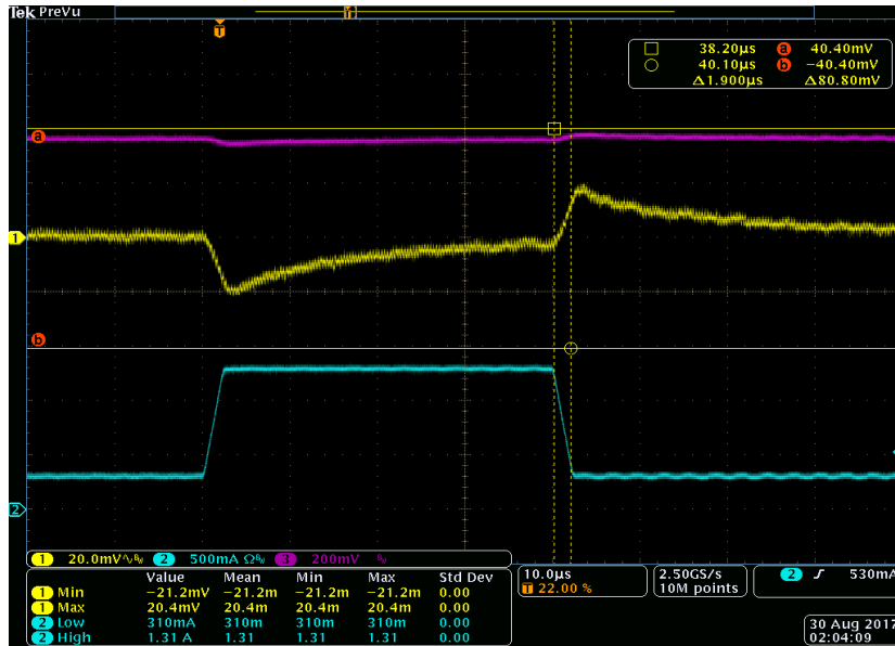
Figure 17: VDDQ (Buck2) Transient Response, V OUT = 1.35 V, 1 A Step
