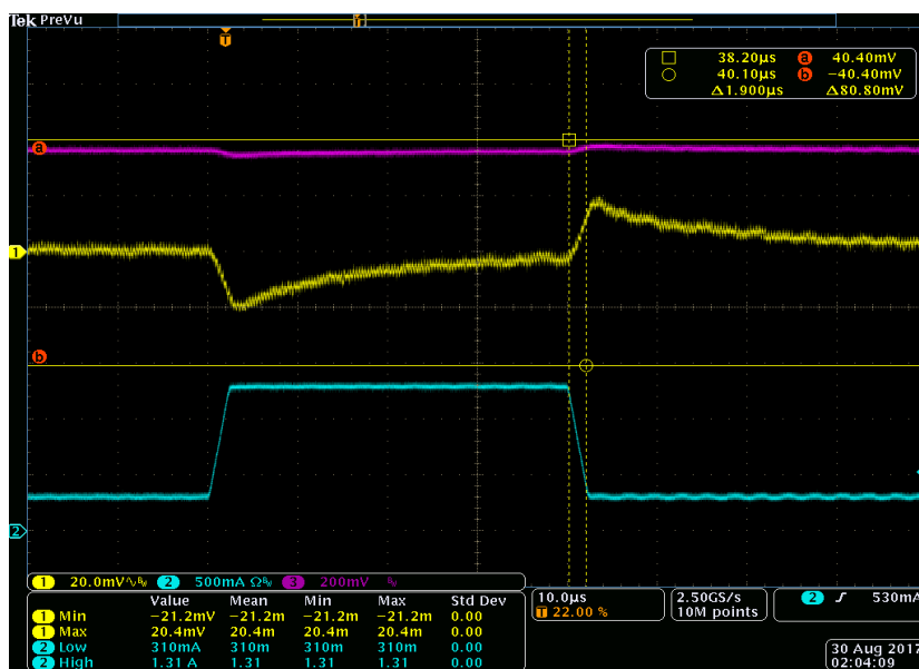
Figure 17: VDDQ (Buck2) Transient Response, V_{OUT} = 1.35 V, 1 A Step
