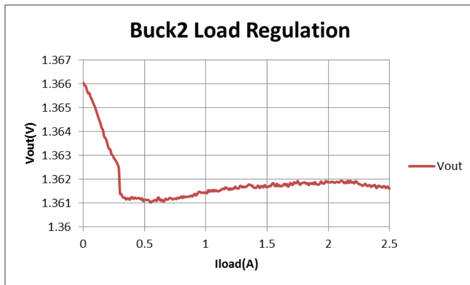
Figure 12: Buck2 Static Load Regulation
