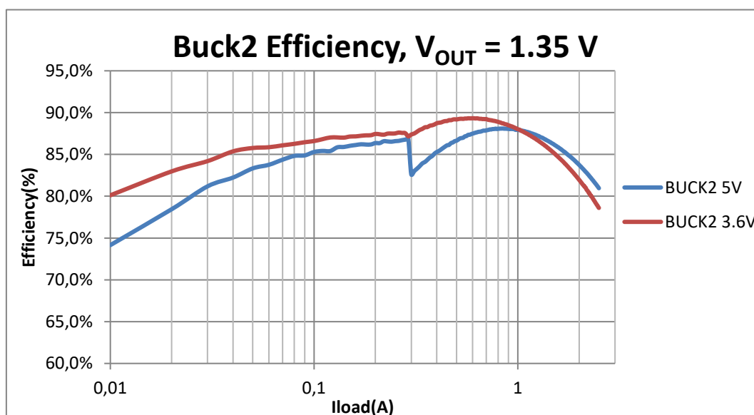
Figure 9: Buck2 Efficiency with V_{OUT} = 1.35\text{ V} and V_{IN} = 5\text{ V} and 3.6\text{ V}
