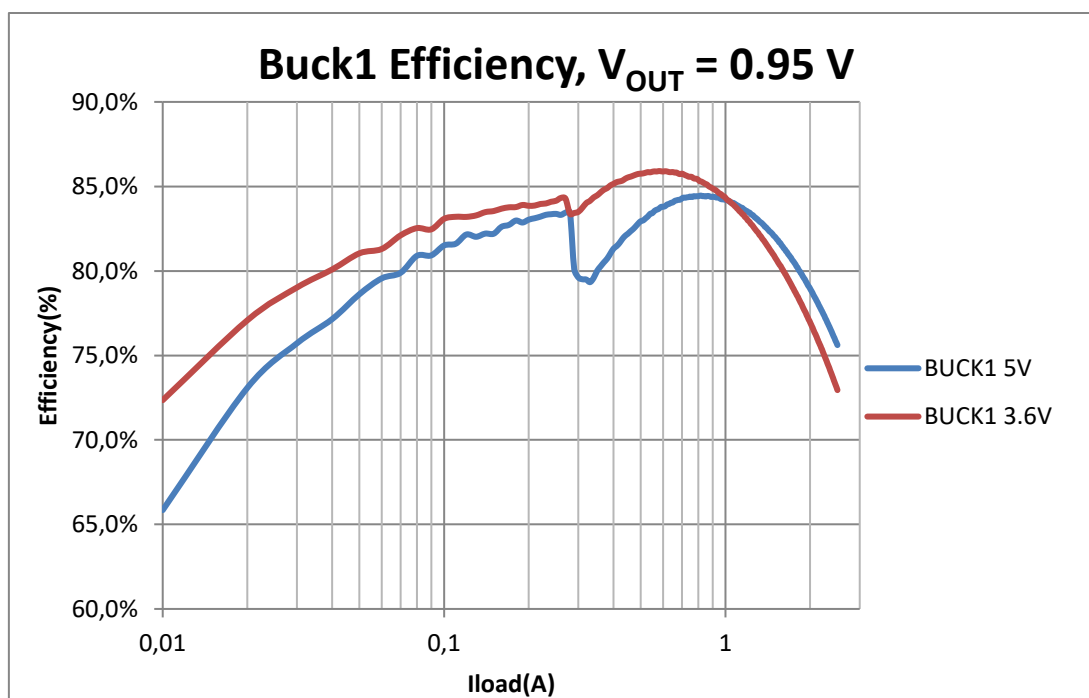
Figure 8: Buck1 Efficiency with V_{OUT} = 0.95\text{ V} and V_{IN} = 5\text{ V} and 3.6\text{ V}
