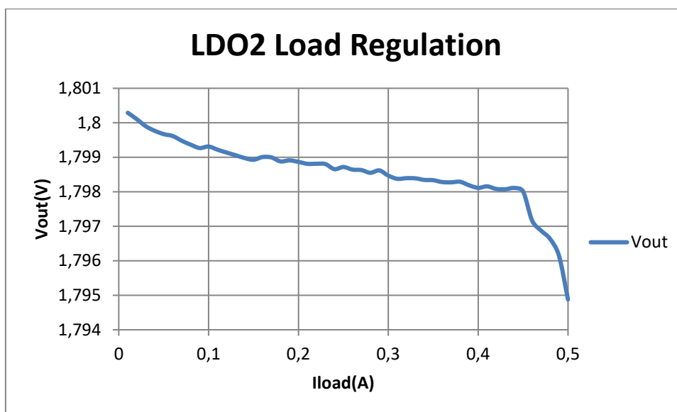
Figure 14: LDO2 Static Load Regulation
