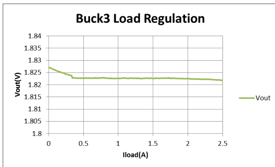
Figure 13: Buck3 Static Load Regulation
