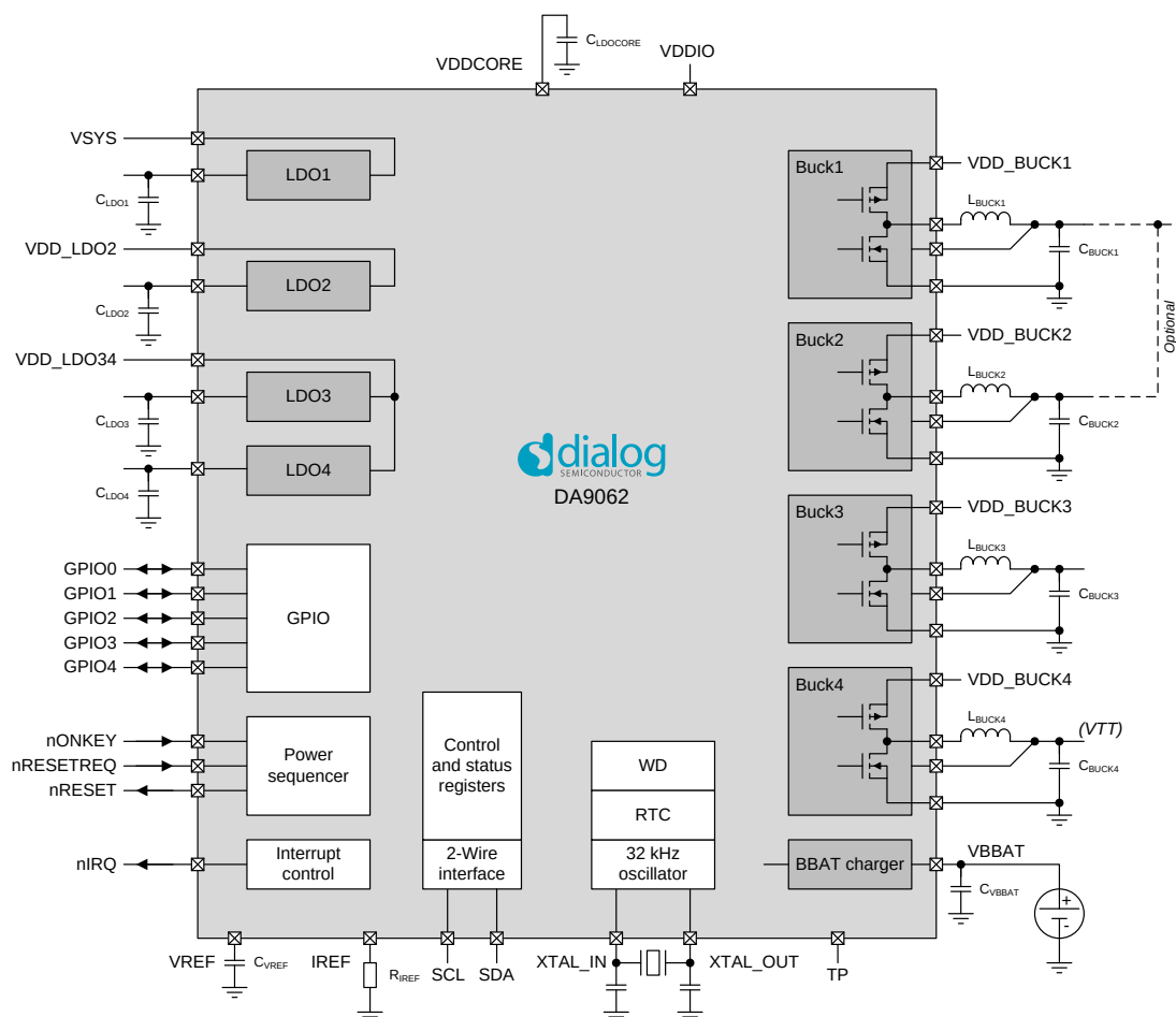
Figure 2: DA9062 Block Diagram
