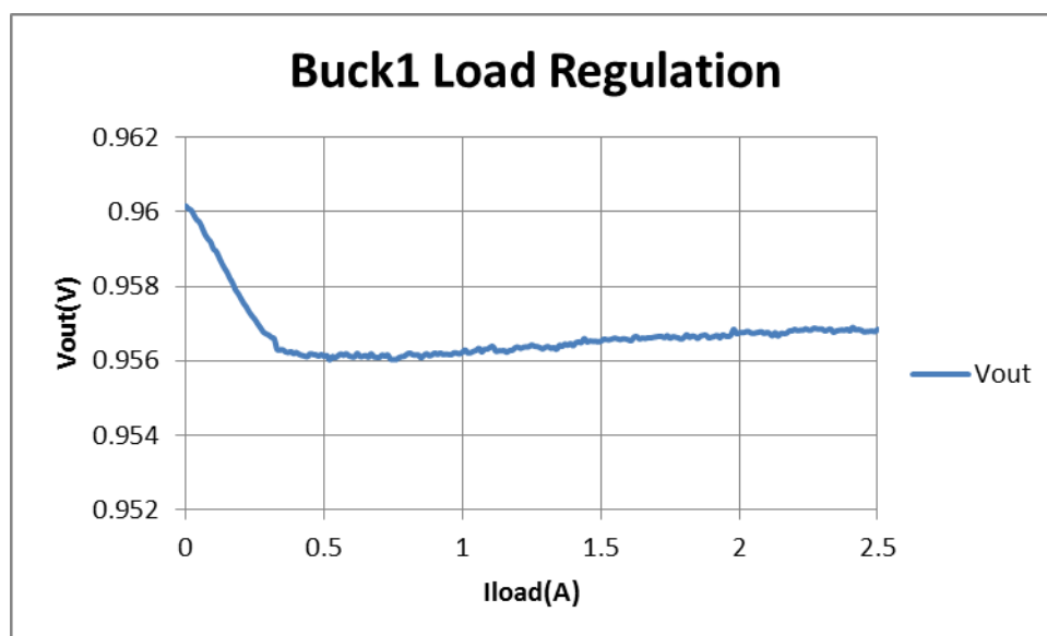
Figure 11: Buck1 Static Load Regulation
