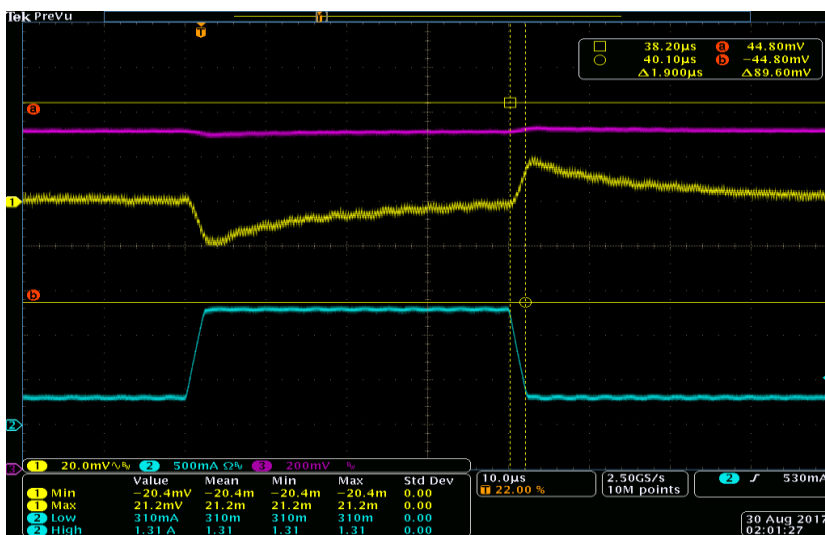
Figure 18: VDDQ (Buck2) Transient Response, V_{OUT} = 1.5 V, 1 A Step
