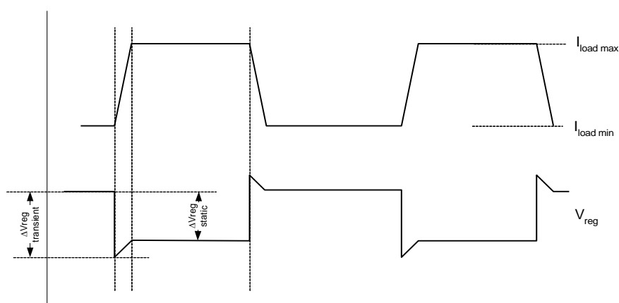
Figure 9: Load regulation
