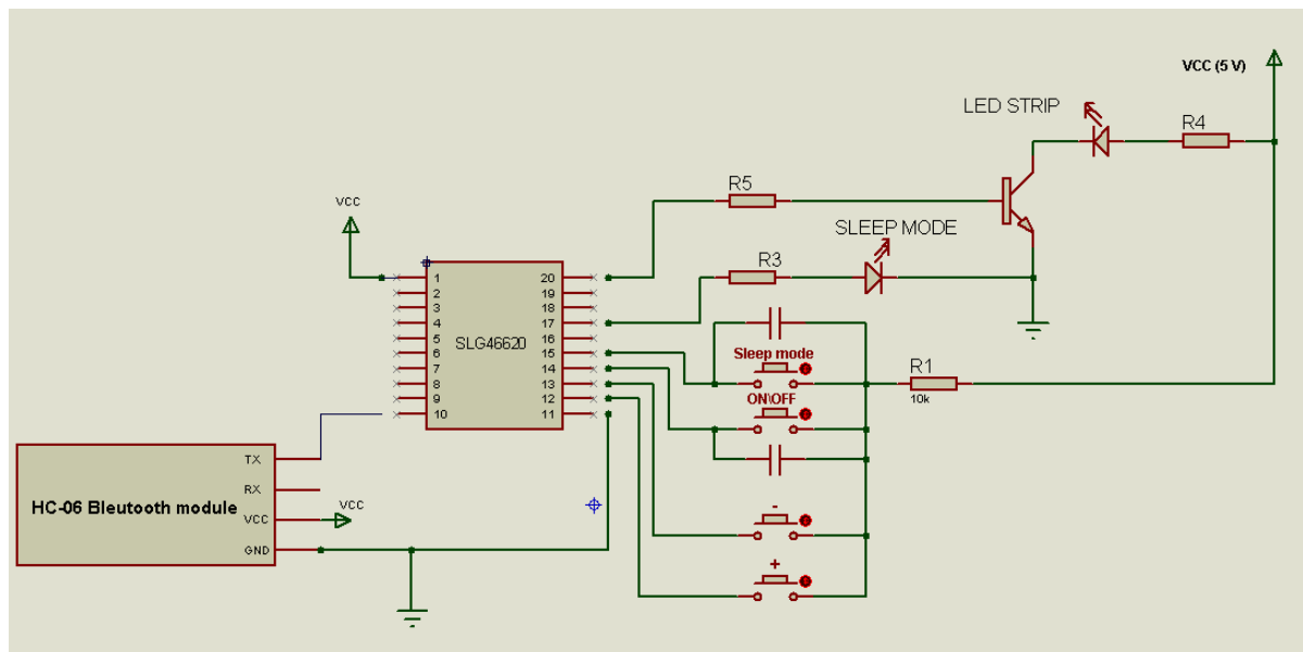
Figure 8: Circuit Schematic
