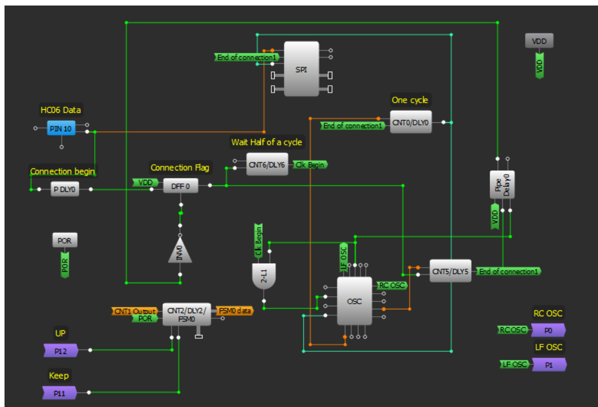
Figure 2: UART Receiver
