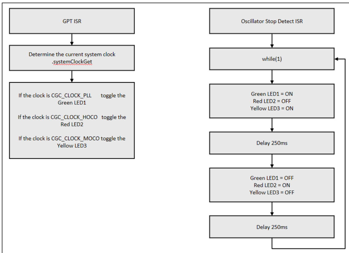
Figure 12. CGC Application Project GPT and Oscillator Stop Detect ISRs
