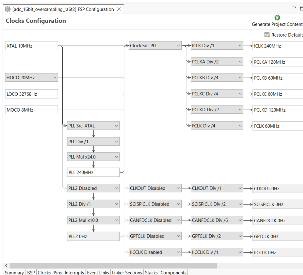
Figure 16. Clock tab of FSP Configuration
