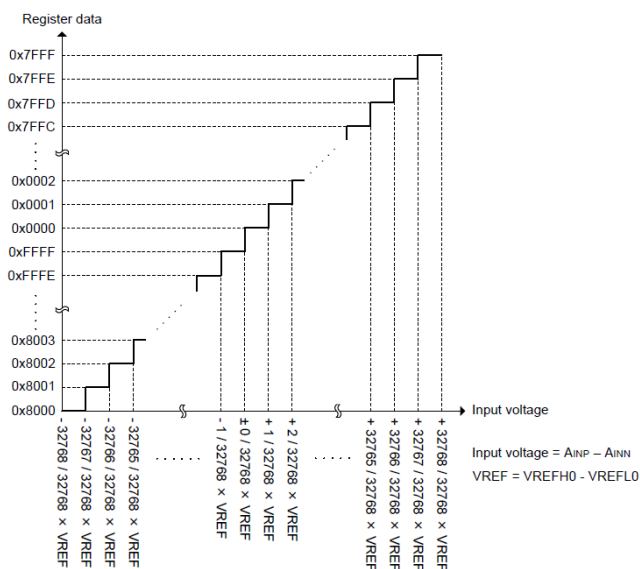
Figure 37. Data Range of A/D Conversion Result (16-bit, signed, differential input)
