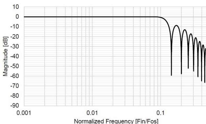
Figure 10. Normalized Frequency Response of the Minimum Phase Filter
