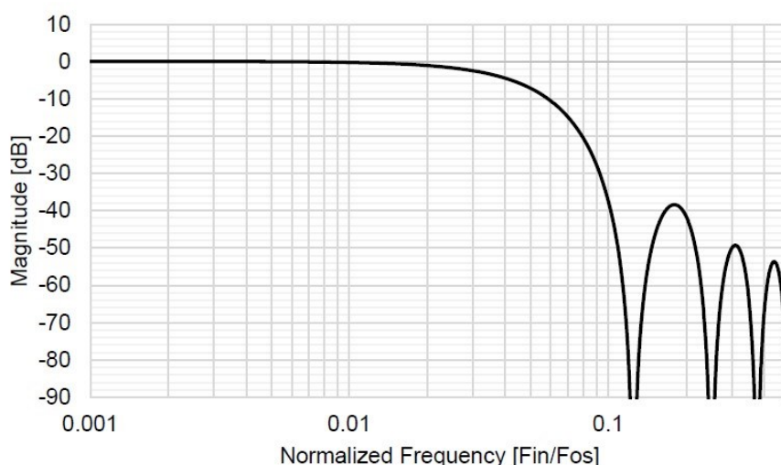
Figure 9. Normalized Frequency Response of the Sinc3 Filter
