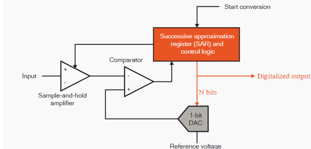
Figure 1. Circuit Block Diagram of SAR ADC
