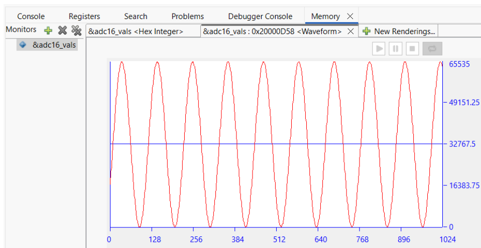
Figure 34. Plot From Running adc_16bit_oversampling_ra6t2 with 250 Hz Input Signal
