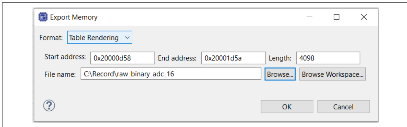
Figure 33. Example of Exporting adc16_vals Array as RAW Binary File
