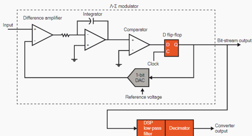
Figure 2. Circuit Block Diagram of Delta-Sigma ADC
