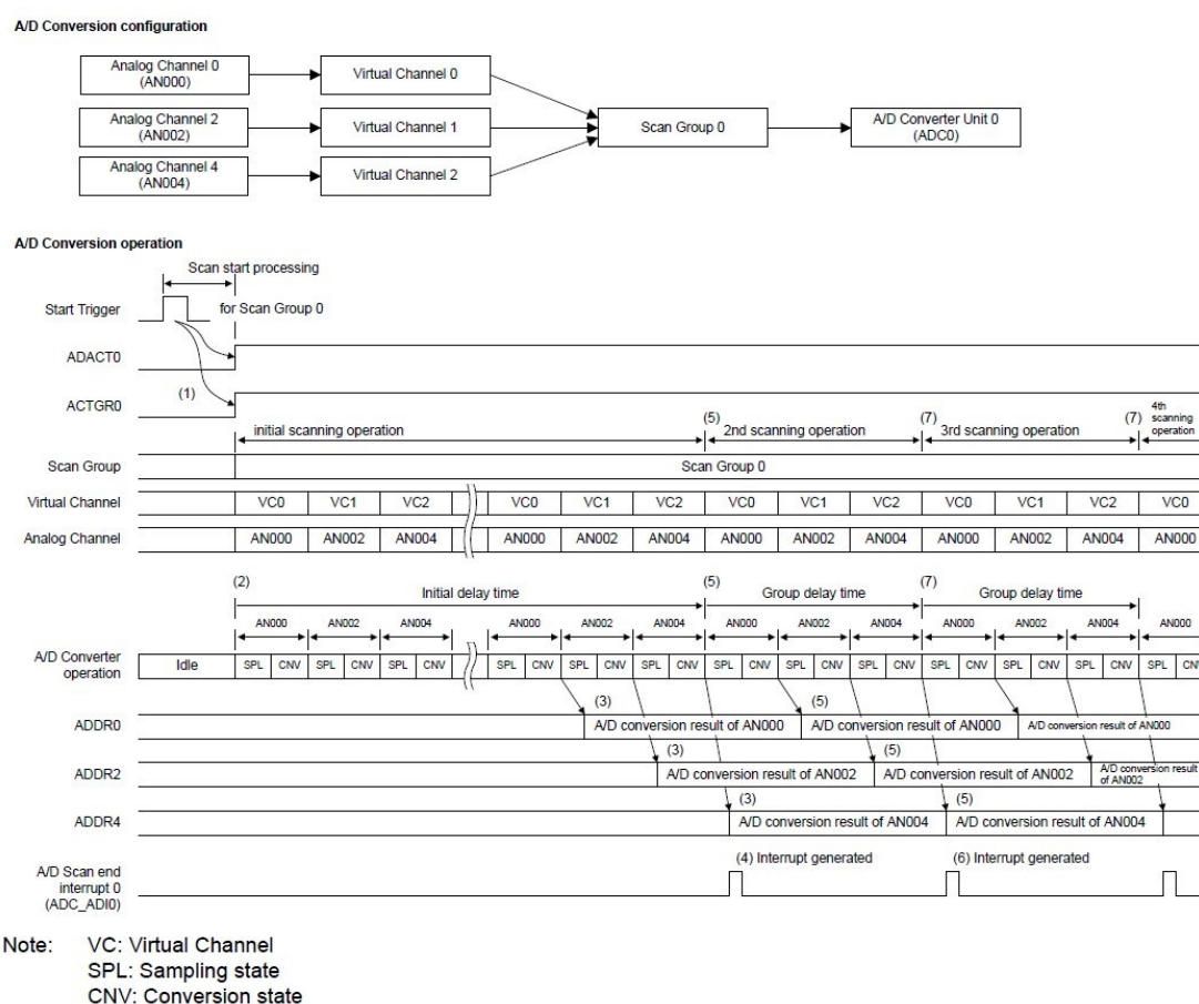
Figure 7. Timing diagram of Hybrid Mode – Continuous Scan Mode
