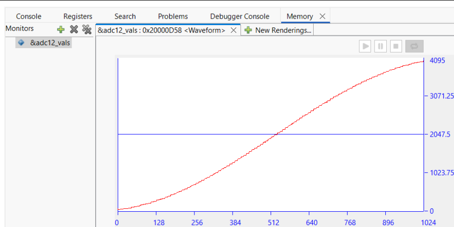
Figure 35. Plot From Running adc_12bit_sar_ra6t2 with 250 Hz Input Signal
