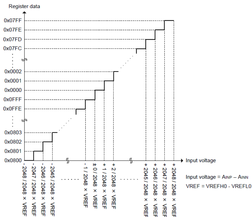
Figure 39. Data Range of A/D Conversion Result (12-bit, signed, differential input)
