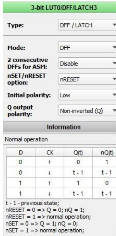
Figure 3. Flip Flop configuration
