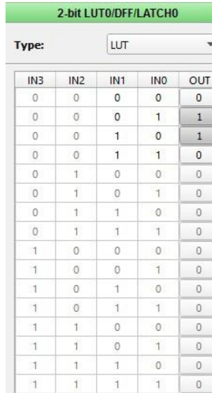
Figure 4. 2-bit LUT configuration
