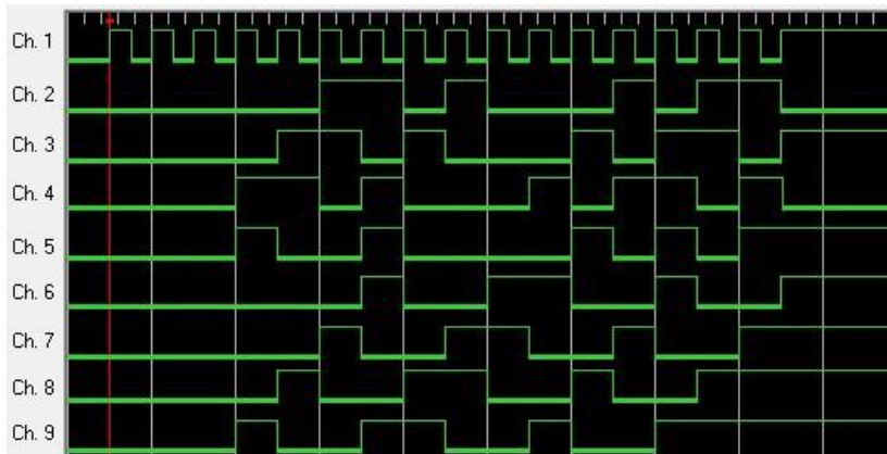
Figure 7. 8-bit 1-wire CRC error code output
