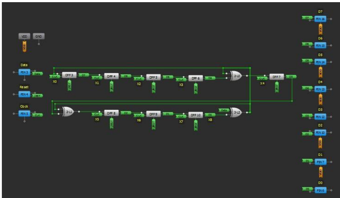
Figure 5. CRC Generator unit block diagram
