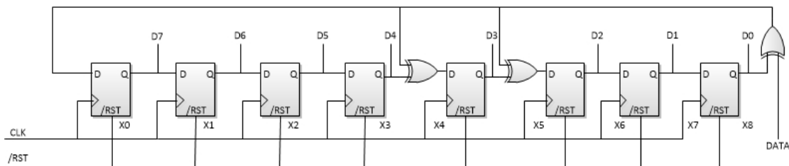
Figure 1. Logic Diagram of 1-Wire CRC Generator Unit
