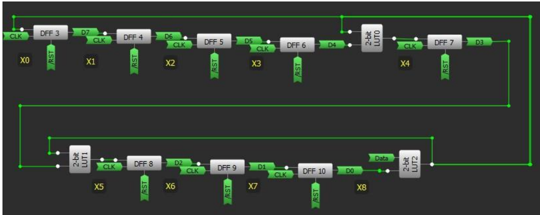
Figure 2. 8-bit Length Shift Register
