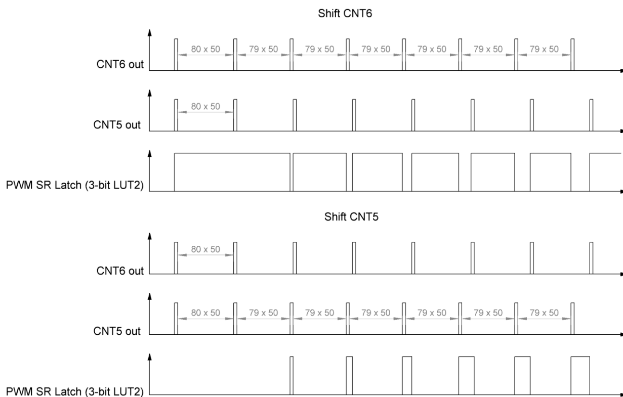
Figure 8. Set and Reset for PWM output
