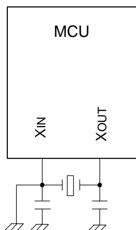
Circuit example (2)
