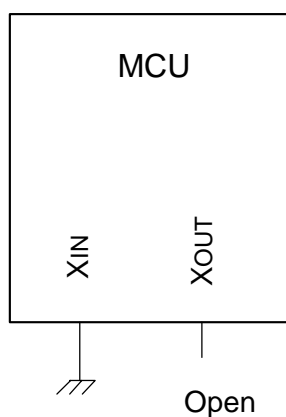
Circuit example (1)
