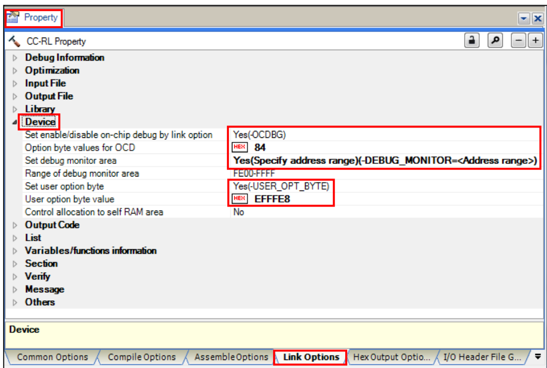
Figure 8-1 (b) Setting of Option byte (CC-RL Compiler)
