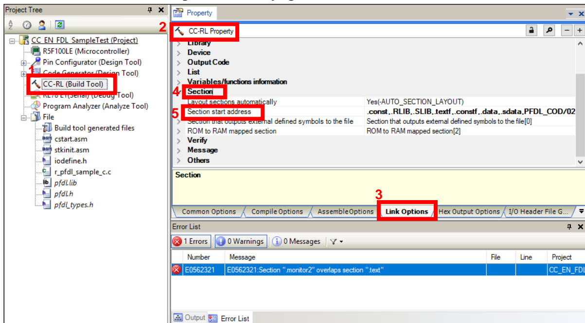
Figure 6-10. Modifying the Section Allocation
