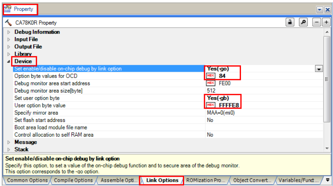
Figure 8-1 (a) Setting of Option byte (CA78K0R Compiler)
