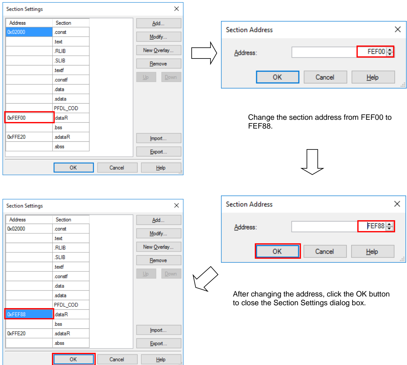
Figure 8-3. Example of Changing the User RAM Area Allocation (RAM Area)
