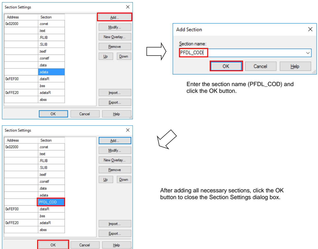
Figure 8-2. Example of Section Settings for the data flash library (ROM Area)
