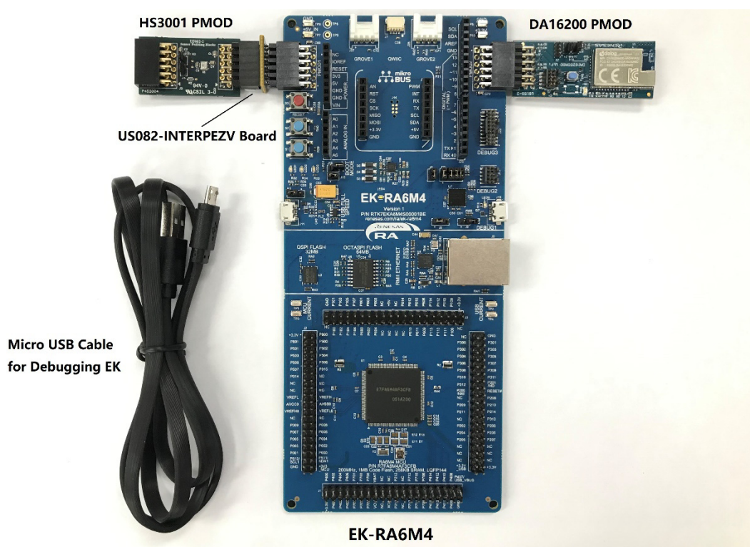
Figure 1. Hardware Components
