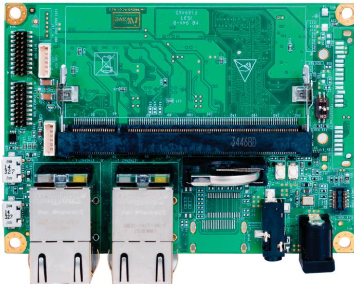
RZ/G1E SODIMM Carrier Card
