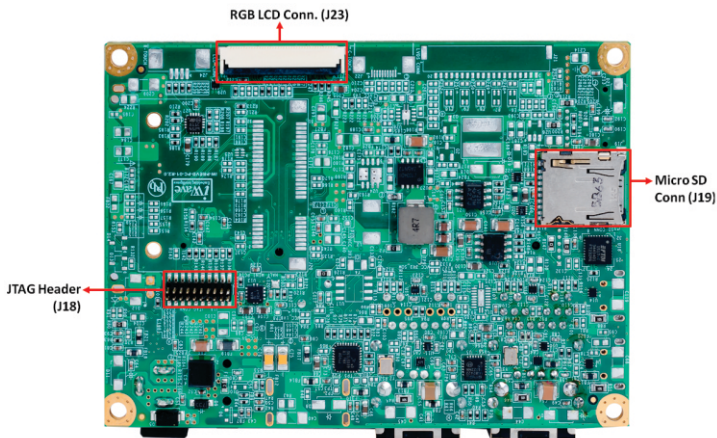
Bottom View of RZ/G1E SODIMM Carrier Card
