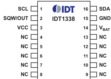
(16-pin SOIC, 300 mil)
