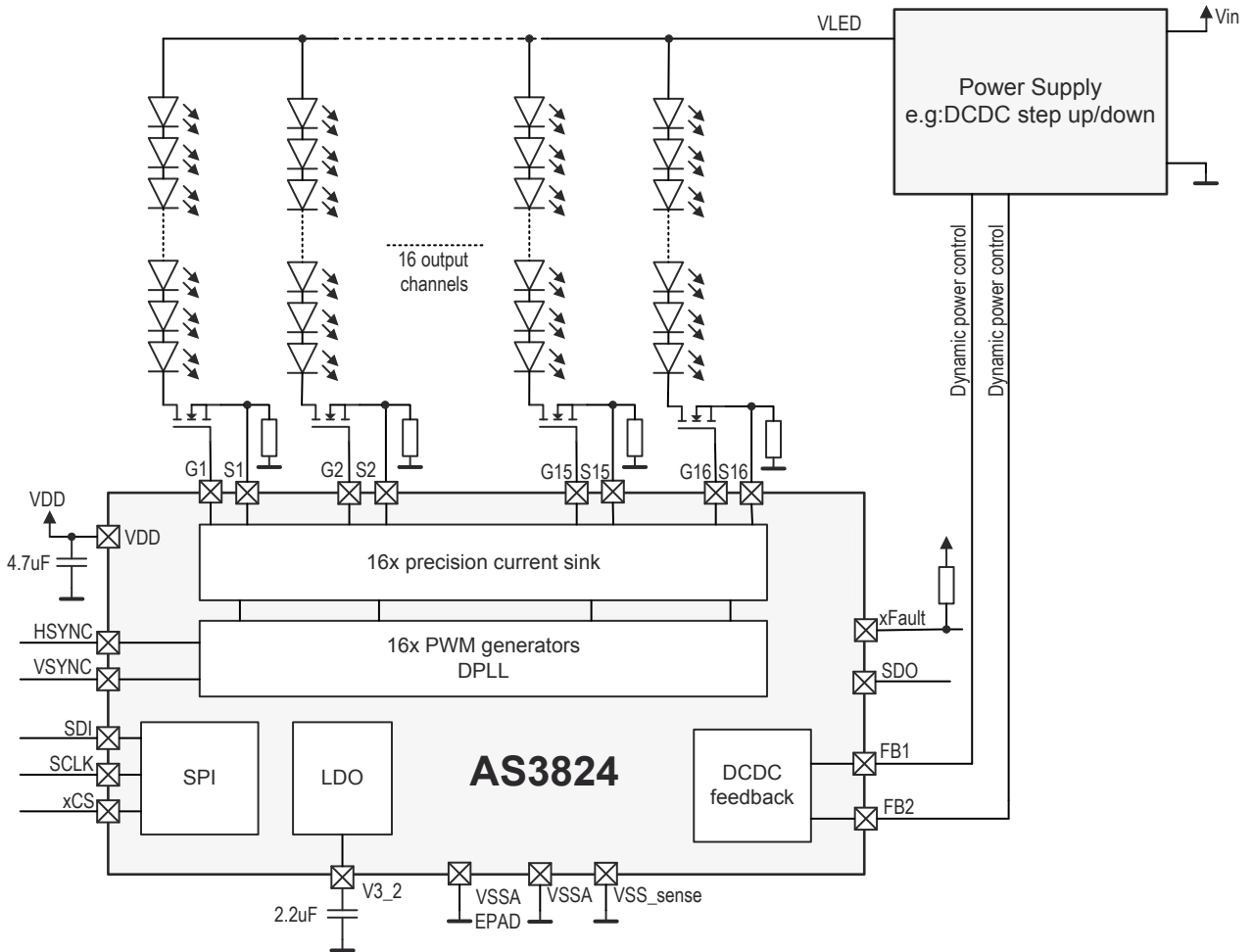
Figure 1. AS3824 Typical Application
