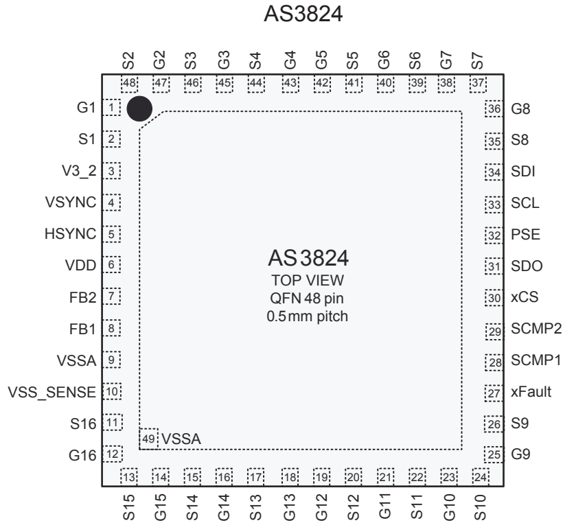
Figure 2. Top View
