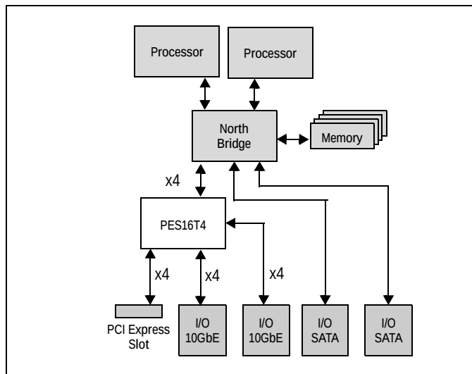
Figure 2 I/O Expansion Application I/O Expansion Application
