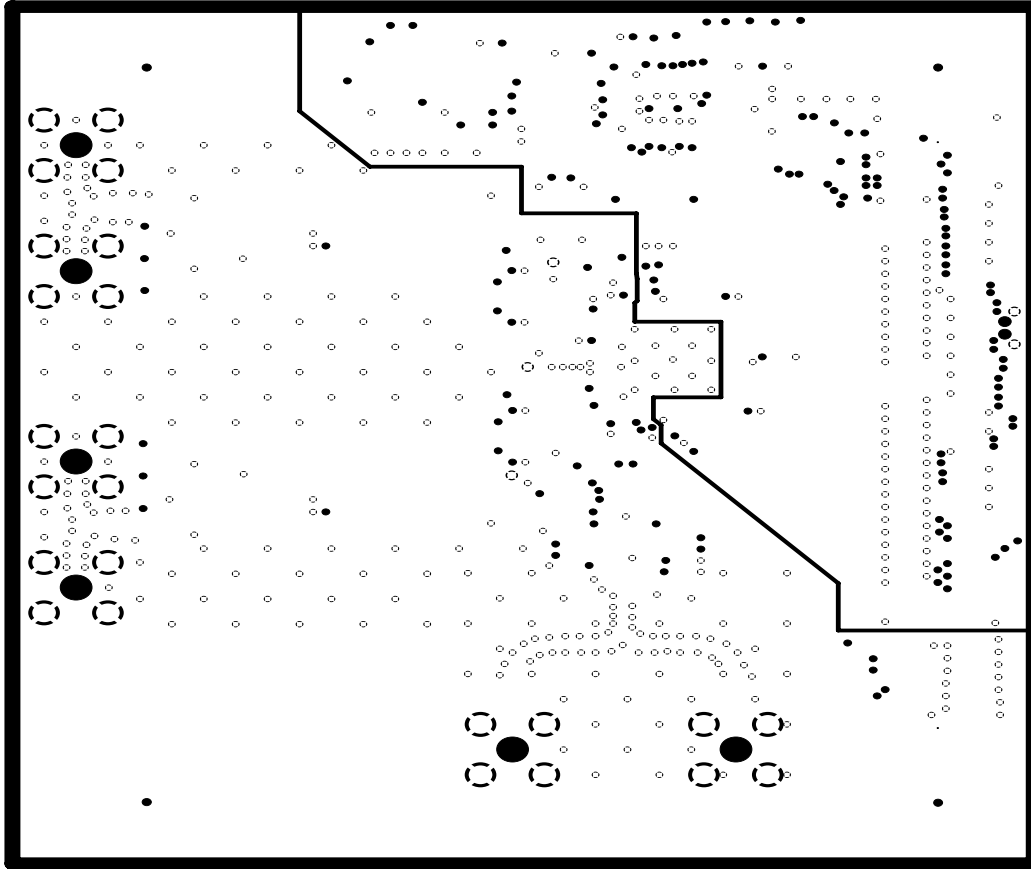
FIGURE 8. GND PLANE 2
