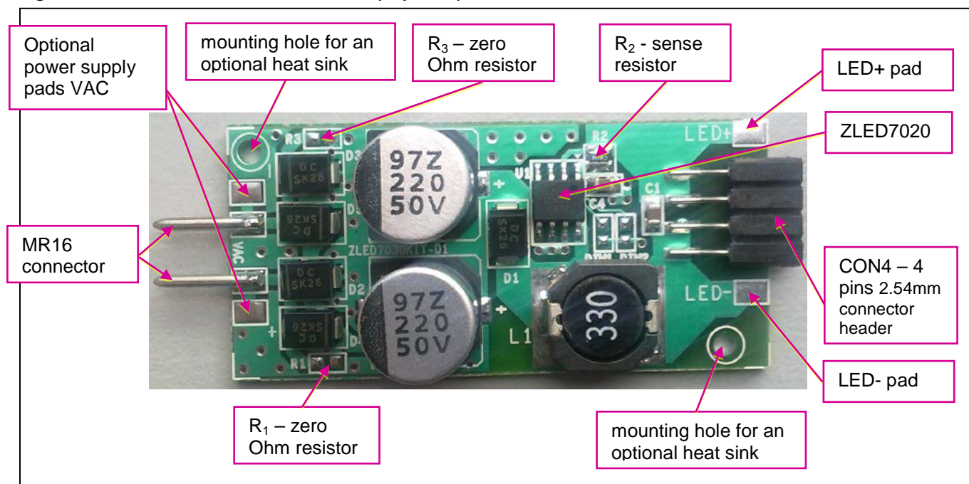
Figure 2.1 ZLED7030KIT-D1 Demo Board (Top View)
