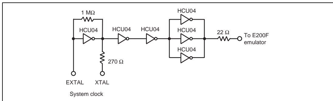
Figure 12 Clock Oscillator
