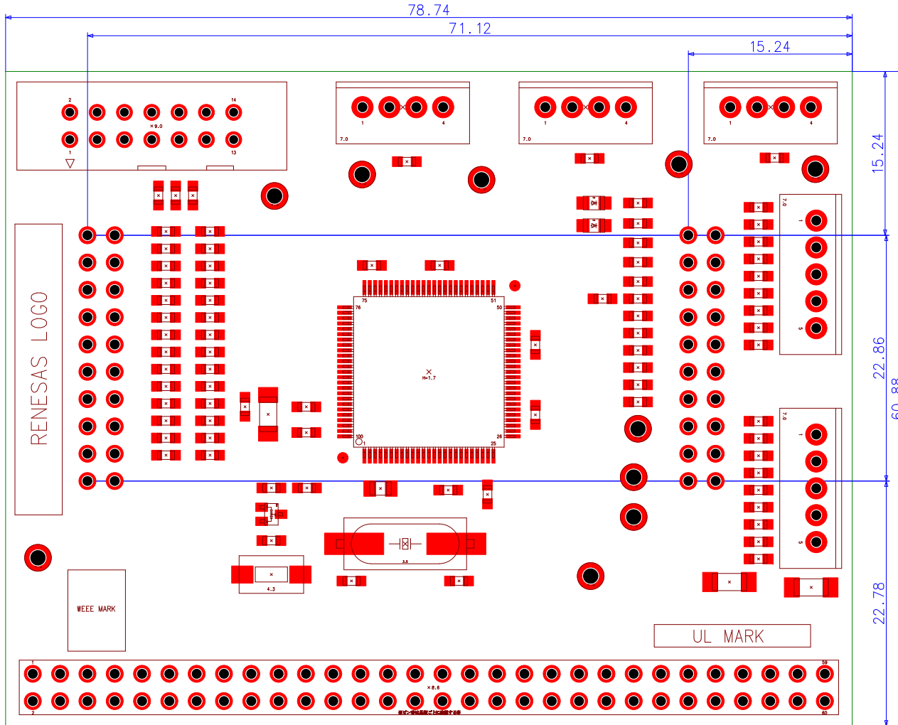
Component side view [Unit : mm]
