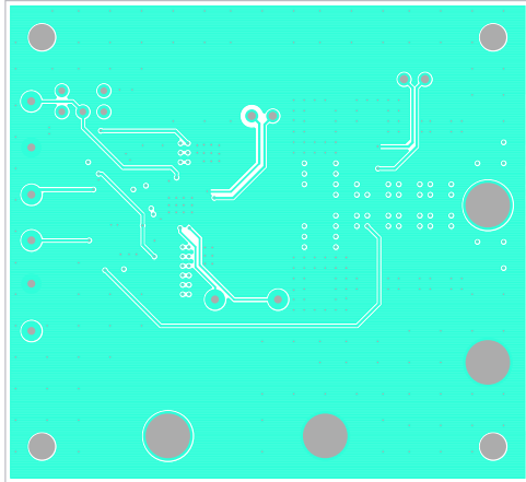
Figure 8. Layer 3
