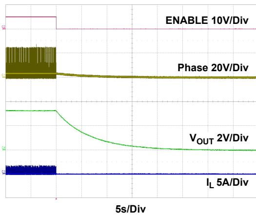
Figure 13. Shutdown through EN, I_{OUT} = 0A
