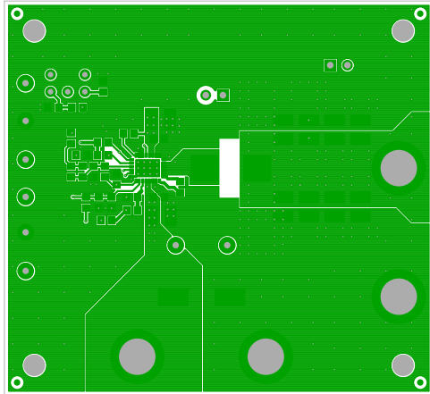
Figure 6. Top Layer
