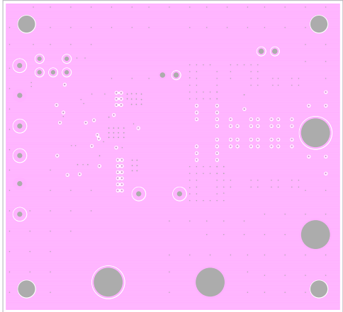
Figure 7. Layer 2
