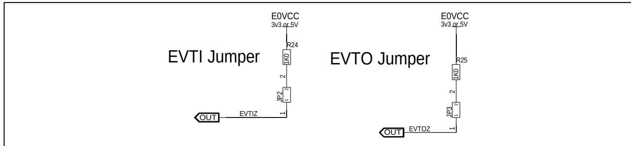
Figure 5.3 EVTI and EVTO jumper
