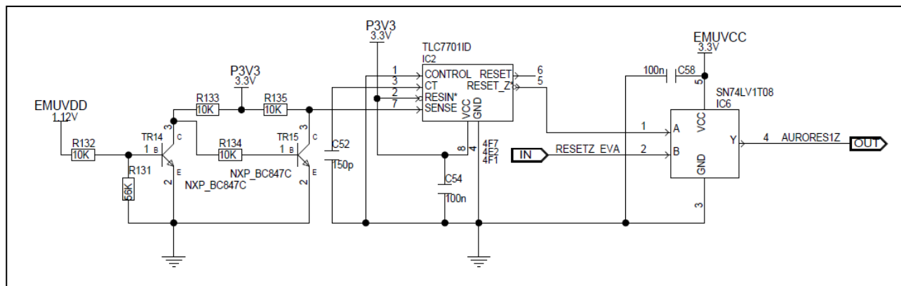
Figure 9.2 AURORES1Z generation board version D016345_06_V01
