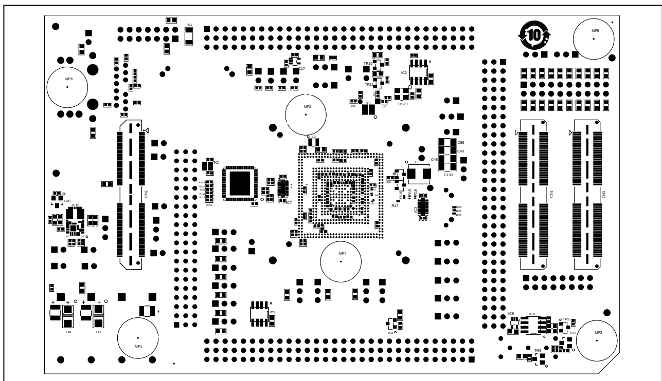
Figure 1.8 D016345_06_V02 Piggyback Board bottom view
