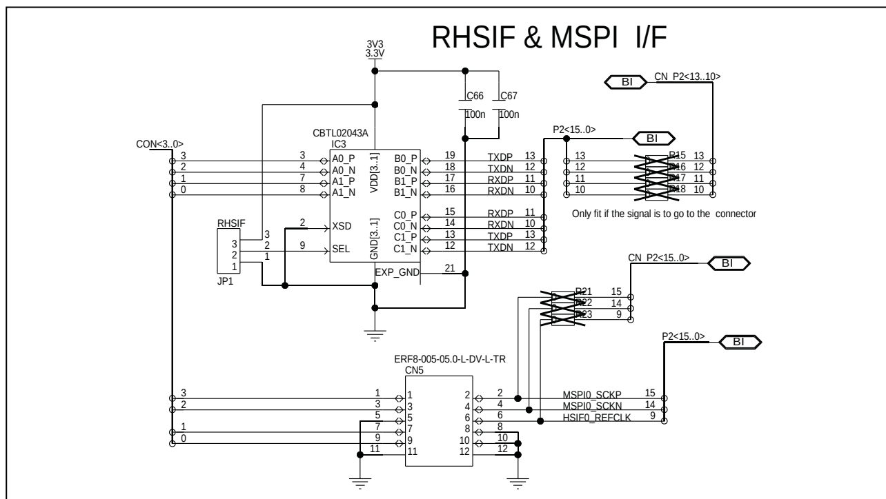
Figure 6.13 RHSIF/MSPI interface on board version D016345_06_V04
