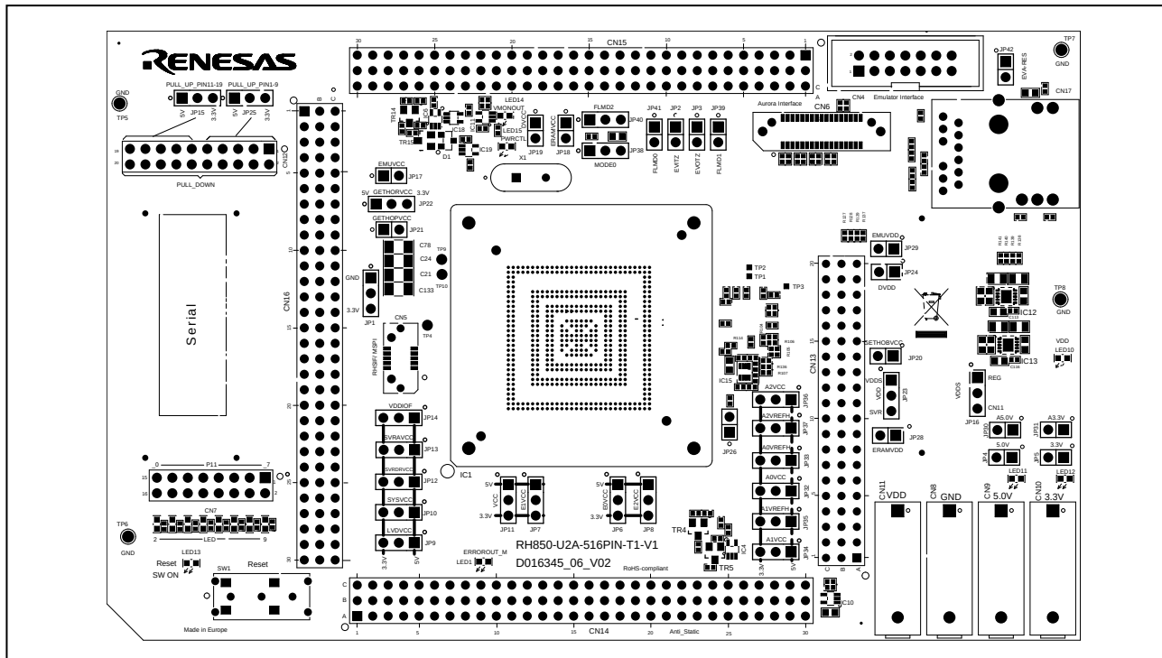
Figure 1.7 D016345_06_V02 Piggyback Board top view
