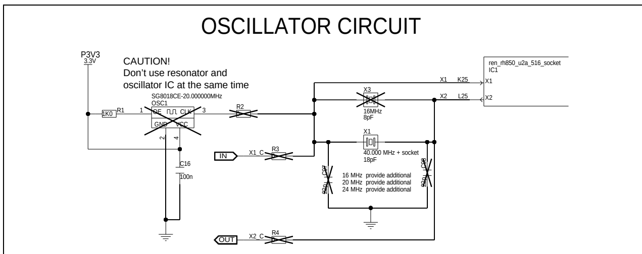
Figure 4.2 Clock supply on board version D016345_06_V03 and D016345_06_V04
