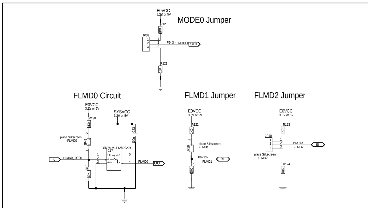
Figure 6.1 Operating mode selection on board version D016345_06_V02
