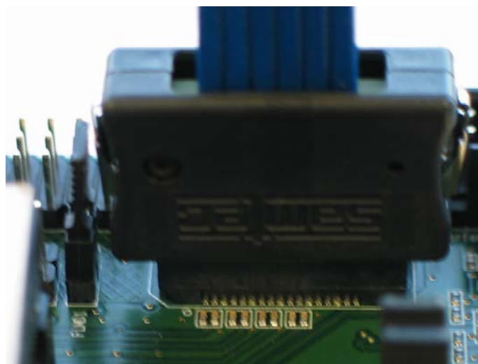
Figure 9.7: OPC displacement of JP39 and CN6 solved new board revision
