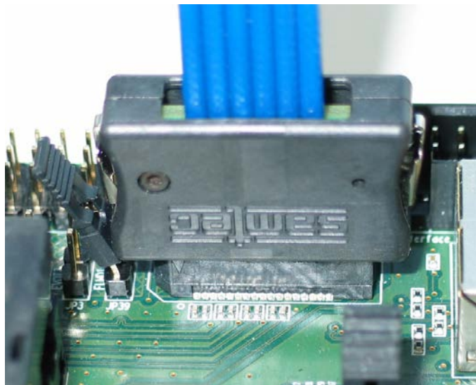
Figure 9.6: OPC displacement of JP39 and CN6
