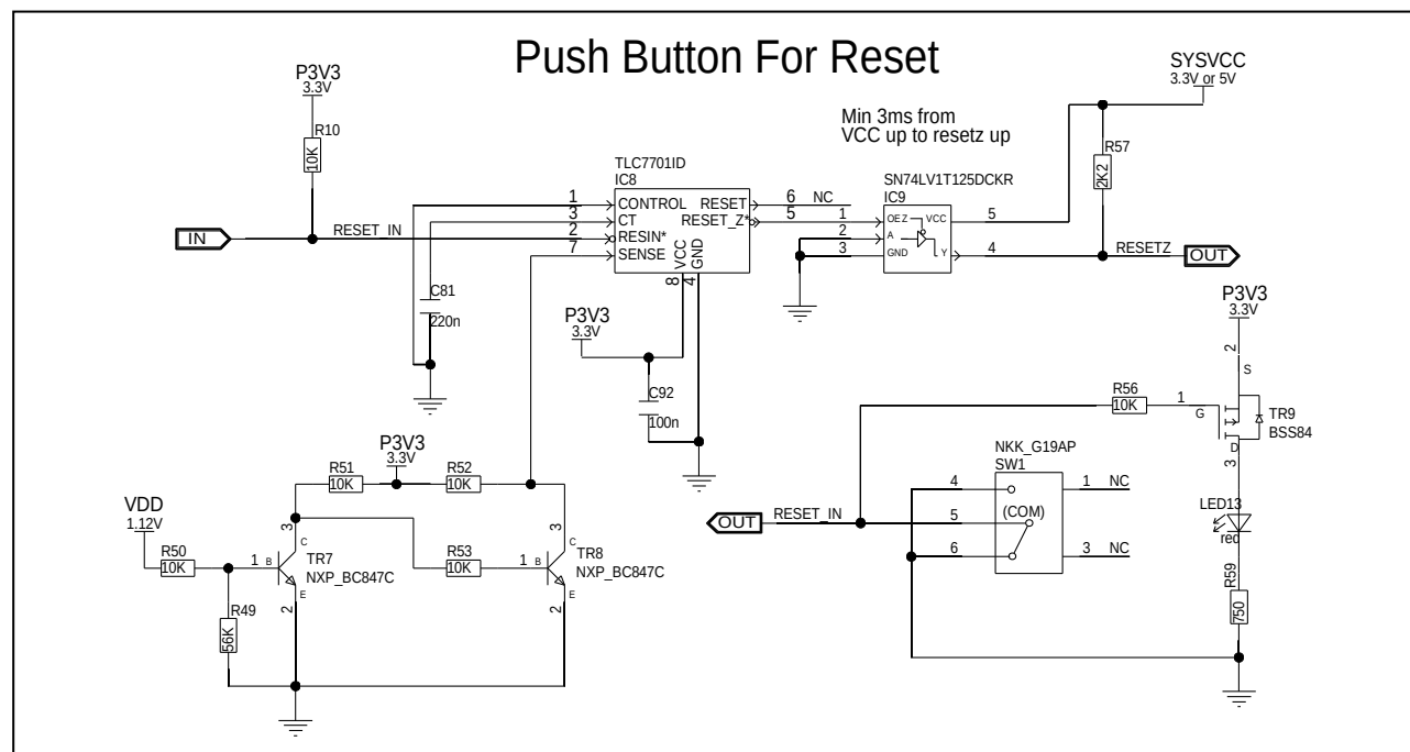
Figure 6.3 RESET circuit on board version D016345 06 V04
