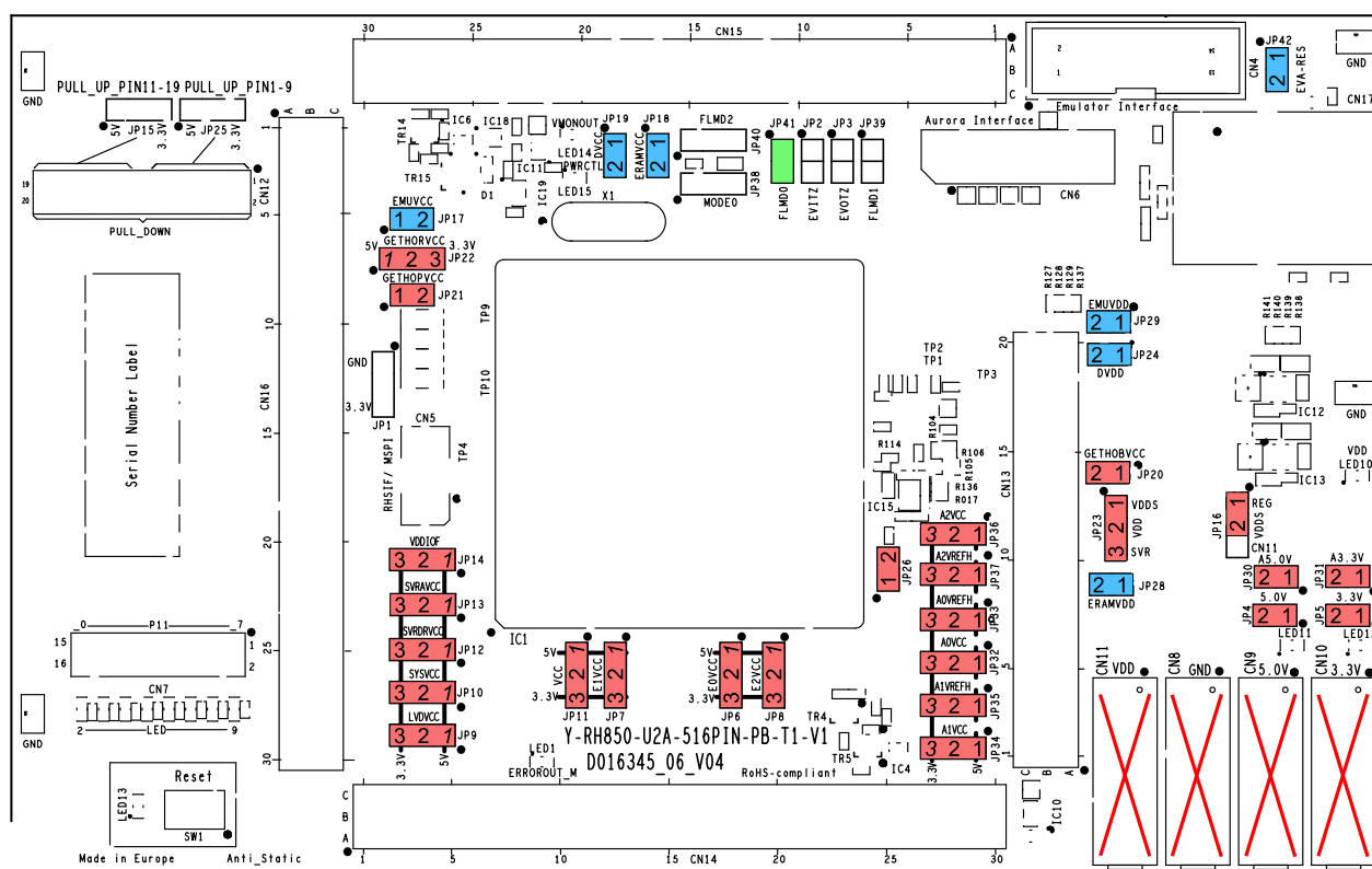
Figure 8.3 Main board operation without external power supply
