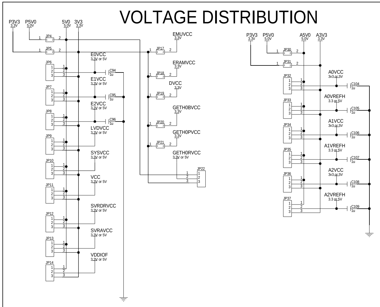
Figure 3.1 Voltage distribution
