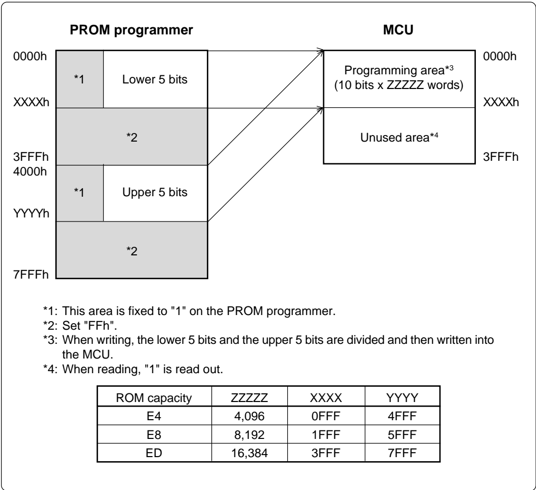
Figure 4.1 Memory maps
