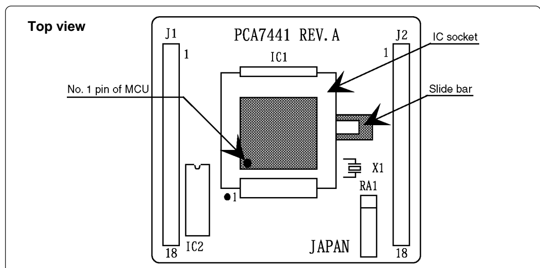
Figure 3.2 Inserting an MCU (PCA7441)
