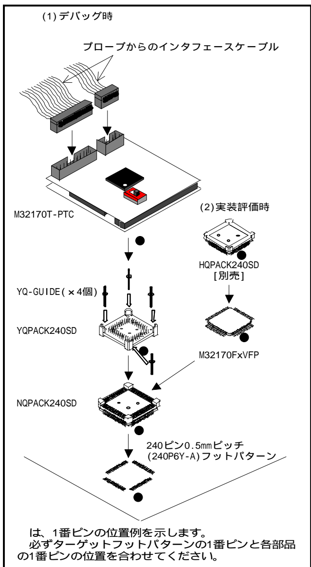
図2 M32170T-PTCの用途
