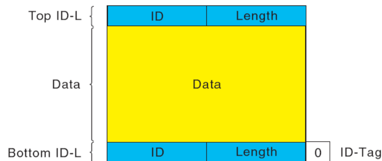
Figure 2 EEPROM Data set representation
