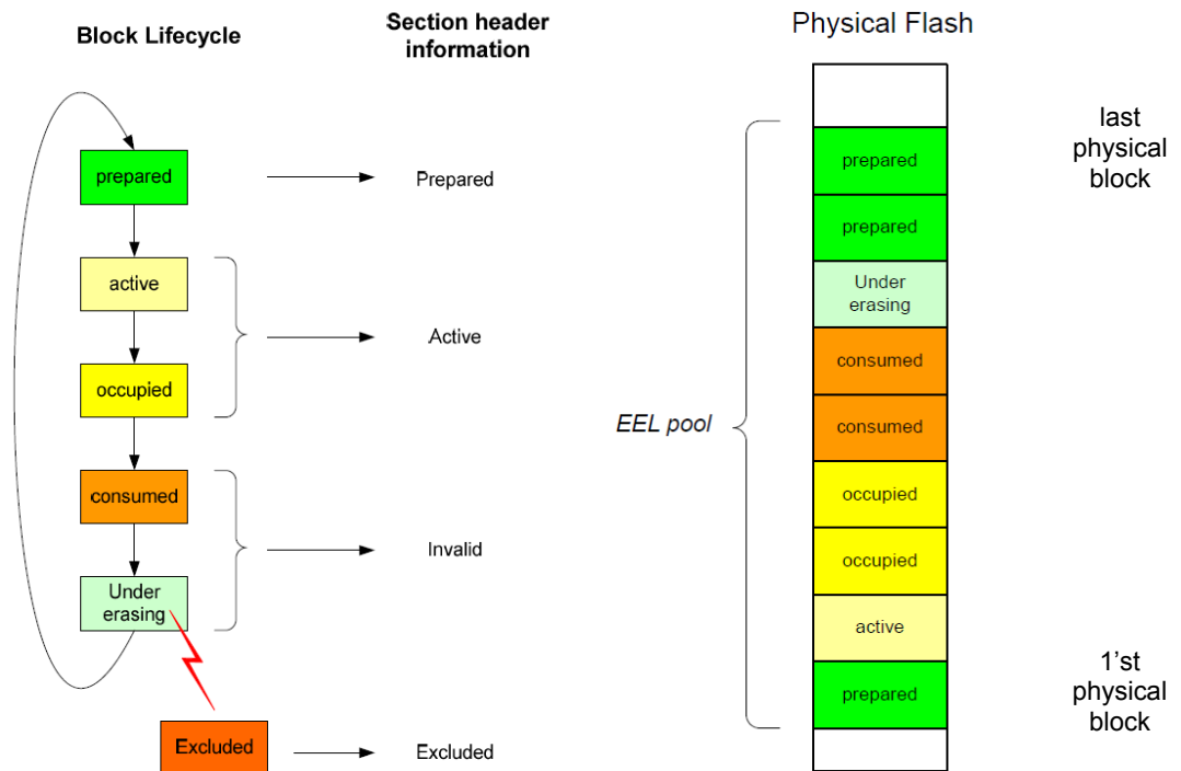
Figure 5 Block Lifecycle & Physical FLASH
