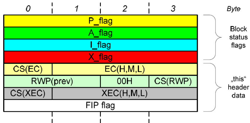
Figure 13 EEL block header structure
