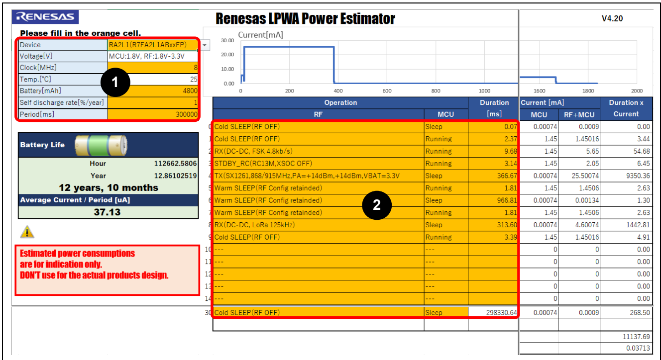
Figure 1. Renesas LPWA Power Estimator GUI
