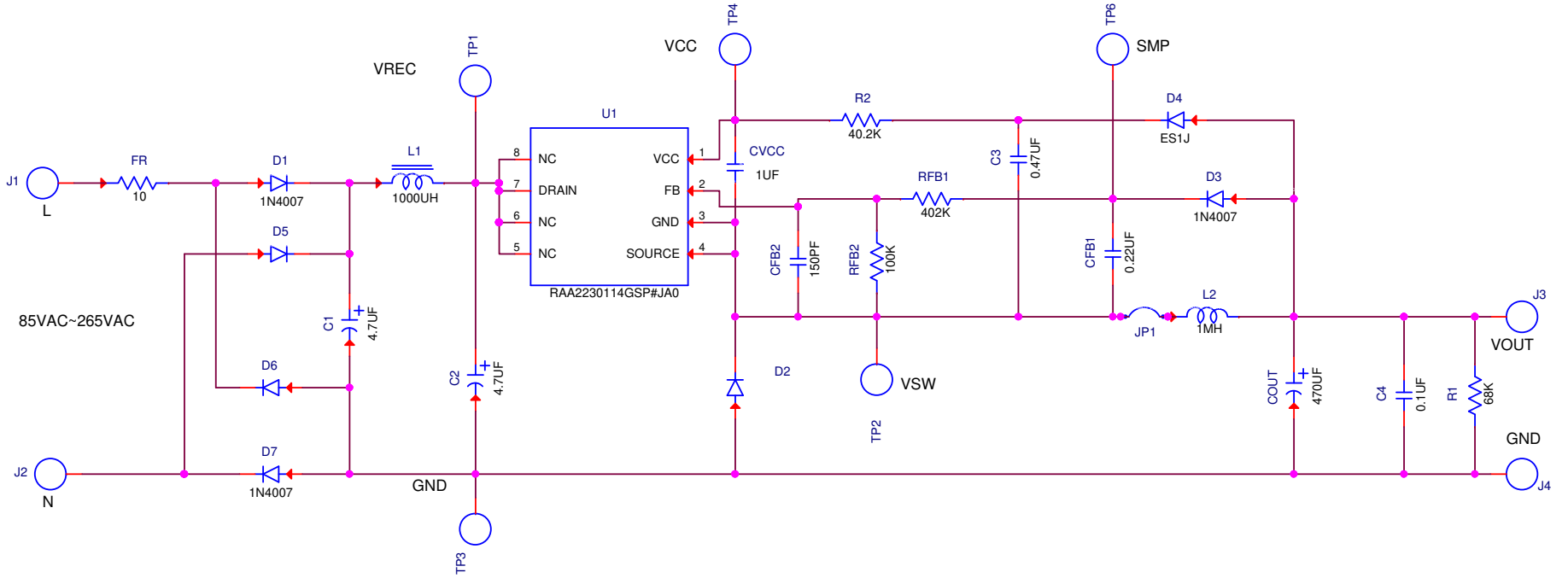
Figure 4. RTKA223011DE0010BU Schematic
