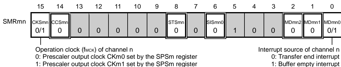
Figure 14-41. Example of Contents of Registers for Master Transmission/Reception of 3-Wire Serial I/O (CSI00) (1/2)
