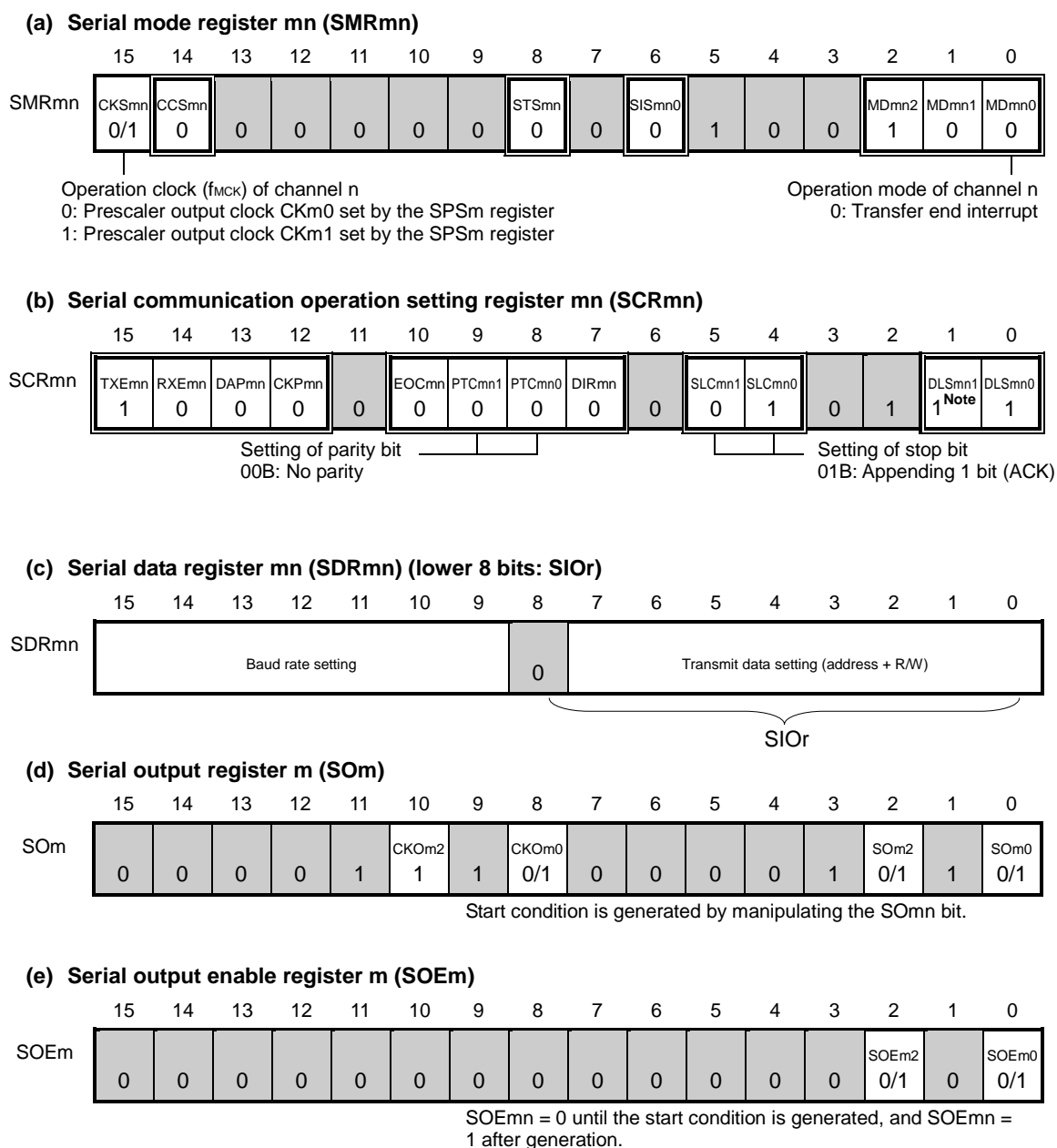
Figure 14-103. Example of Contents of Registers for Address Field Transmission of Simplified I 2 C (IIC00, IIC10) (1/2)
