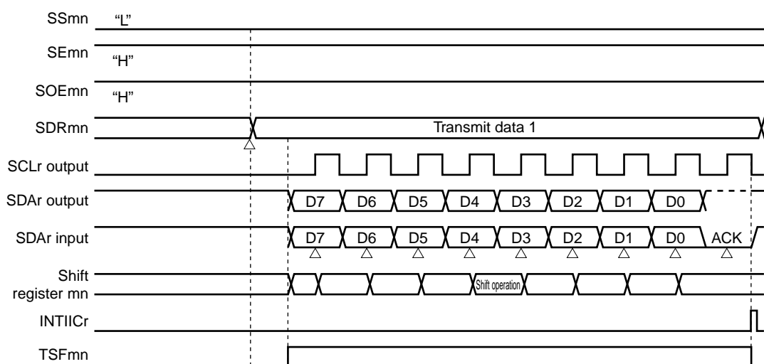
Figure 14-108. Timing Chart of Data Transmission
