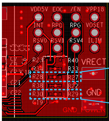
Figure 8. Locations of R27, R28, R29, and R30 on the PCB
