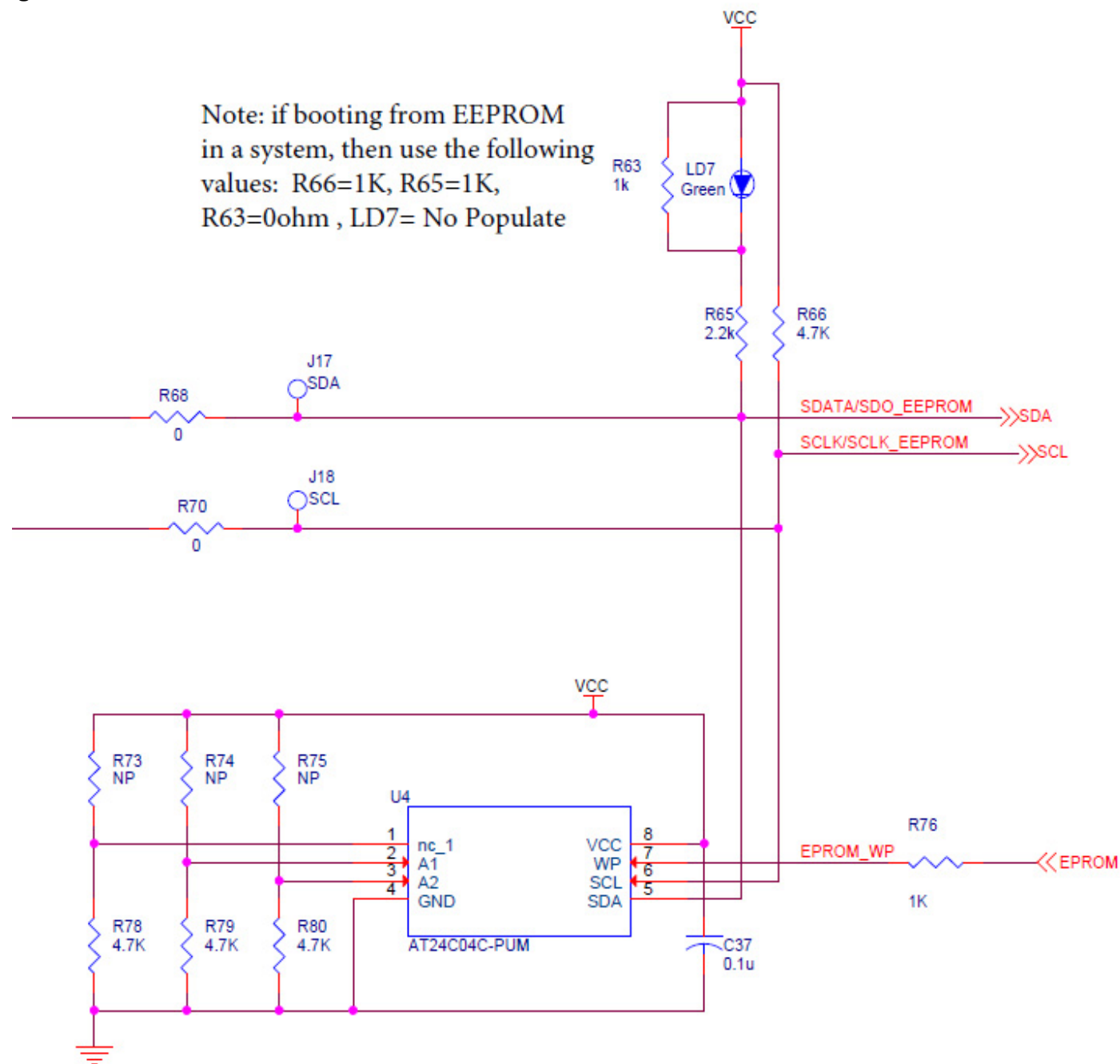
Figure 6. EEPROM/I2C Schematic
