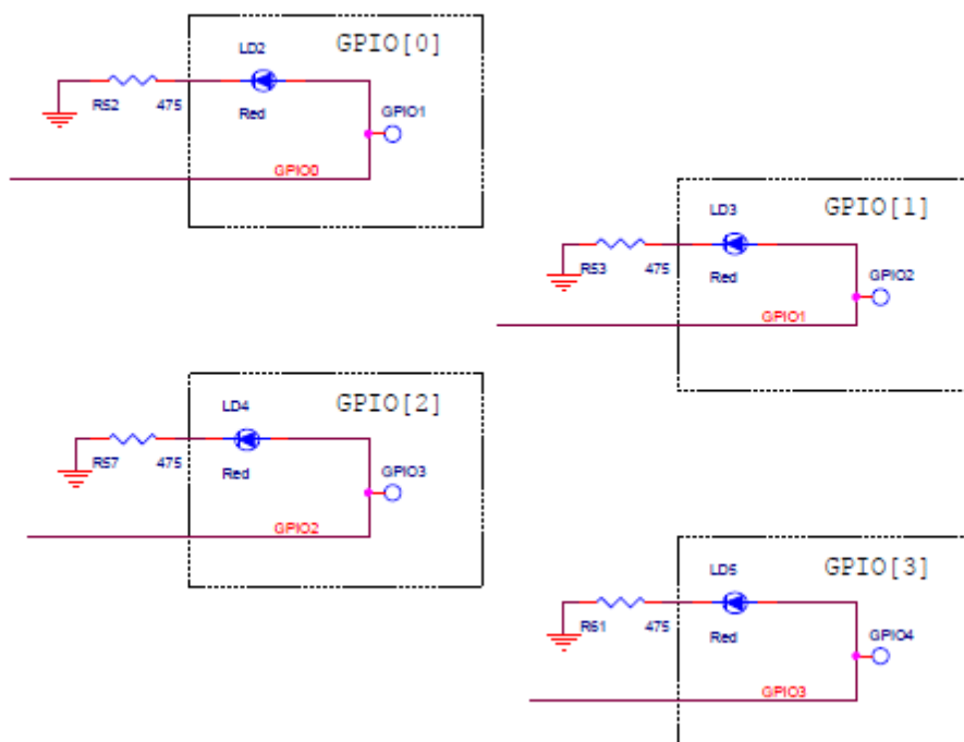
LED on= logic 1
