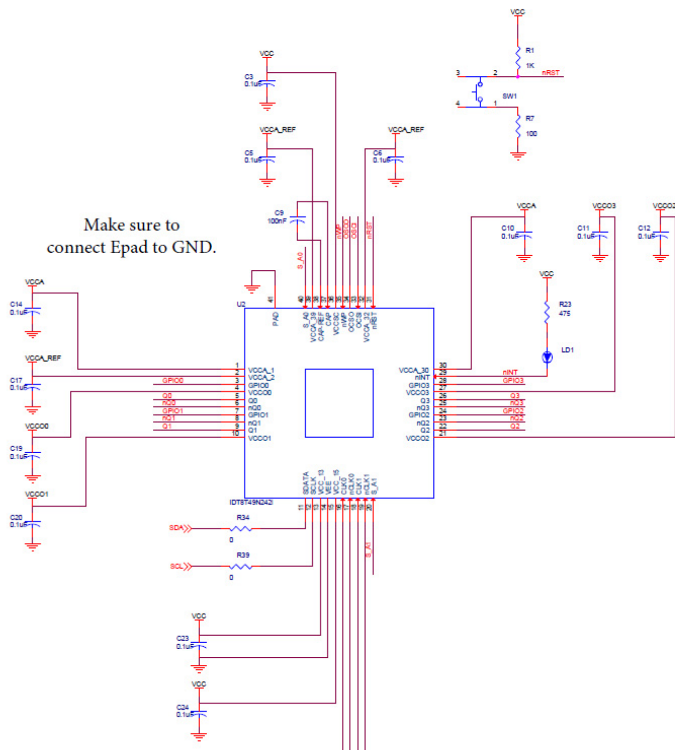
Figure 11. 8T49N241 and 8T49N242 DUT Schematic
