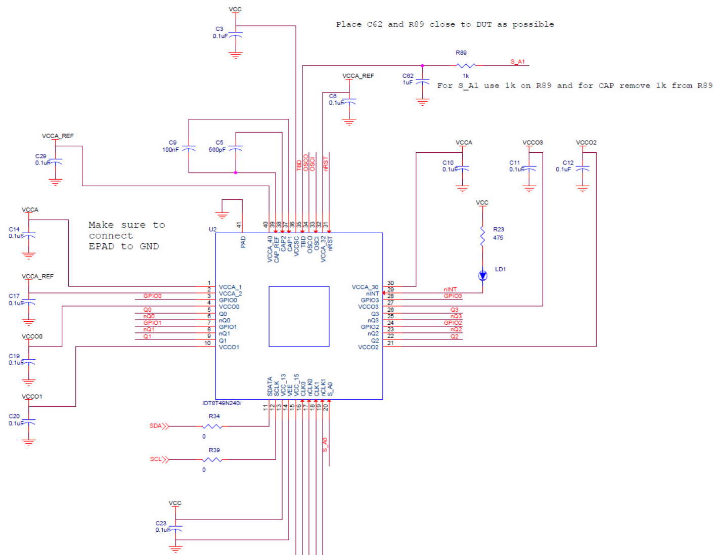
Figure 12. 8T49N240 DUT Schematic
