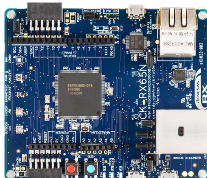
CK-RX65N
