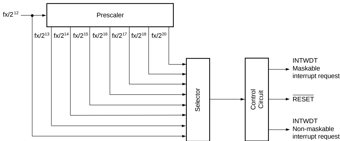
Figure 5-10: Watchdog Timer Block Diagram
