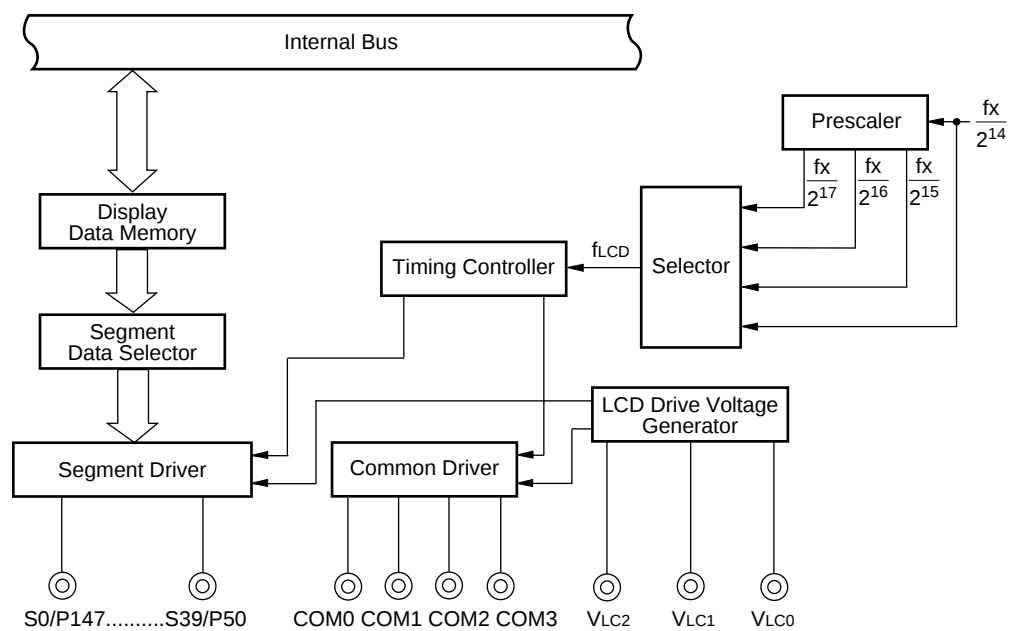
Figure 5-20: LCD Controller/Driver Block Diagram
