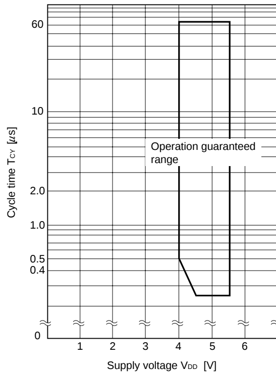
Figure 12-1: T_{CY} vs V_{DD} (At f_x = f_x/2 main system clock operation)
