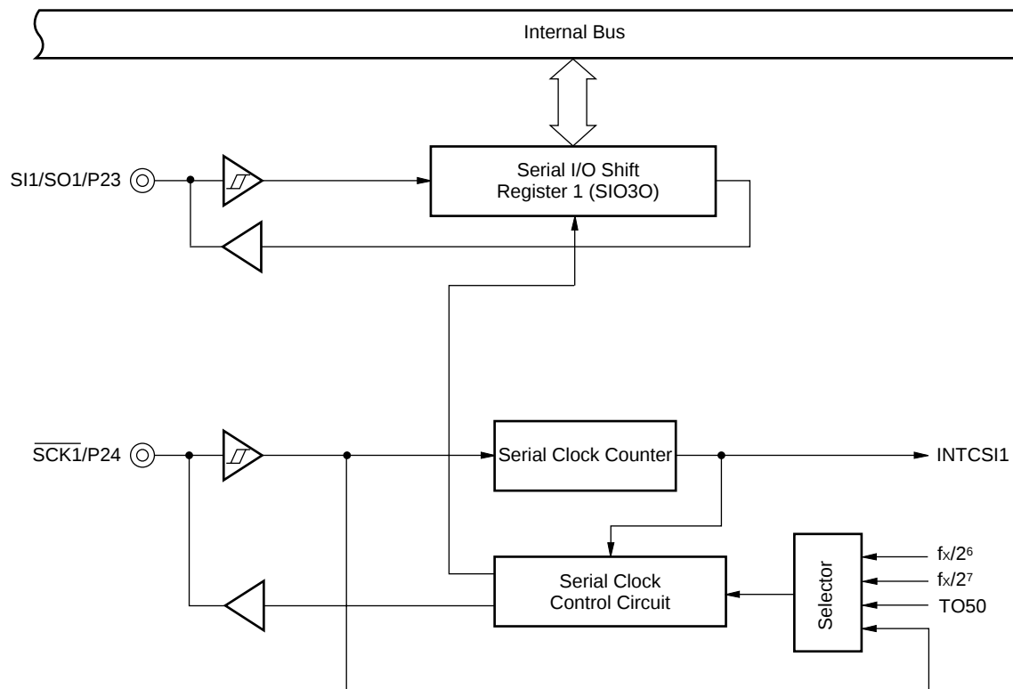
Figure 5-17: Serial Interface Channel 1 Block Diagram
