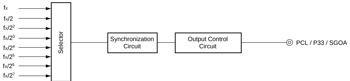
Figure 5-11: Clock Output Control Circuit Block Diagram
