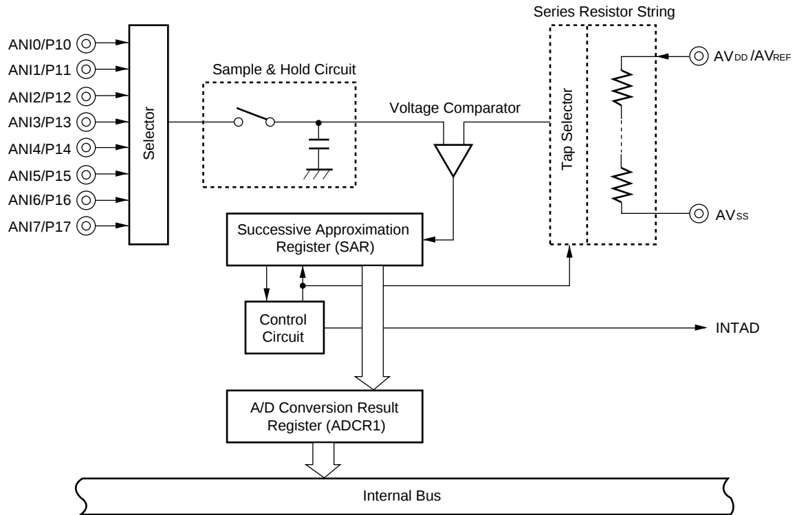
Figure 5-14: A/D Converter Block Diagram
