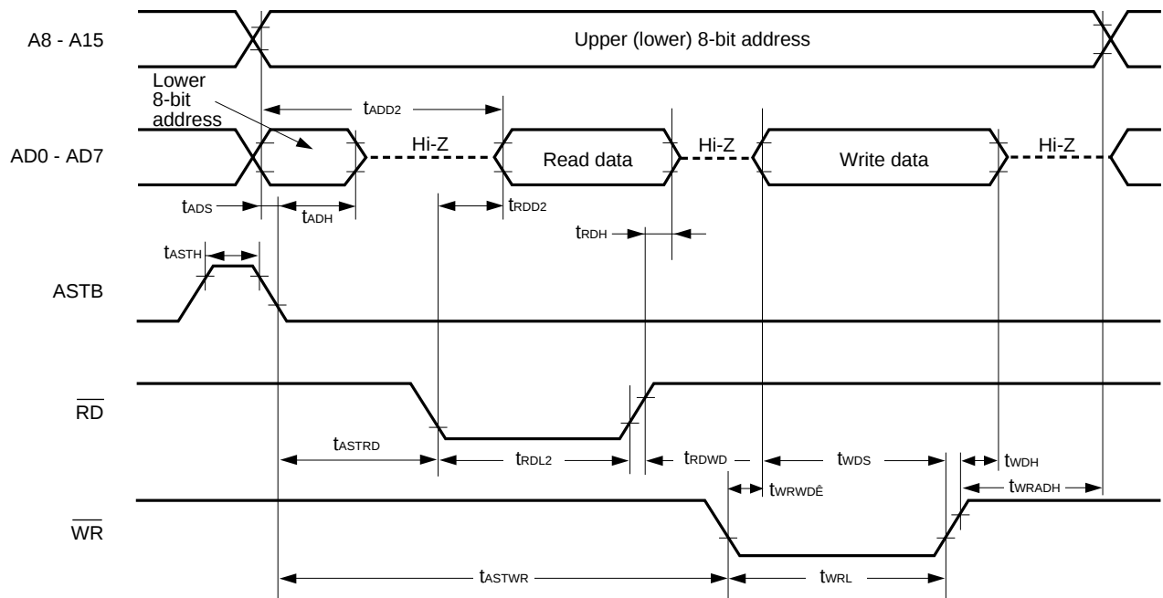
Figure 12-7: External data access (no wait)
