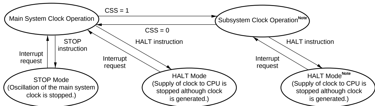
Figure 9-1: Standby Function
