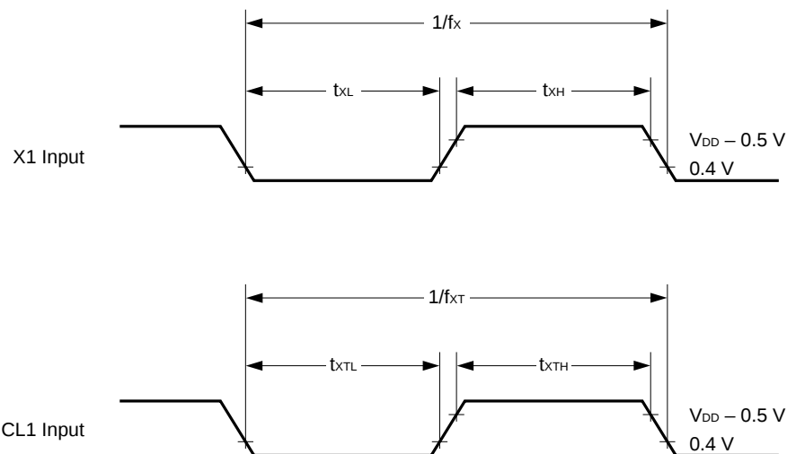
Figure 12-3: Clock Timing
