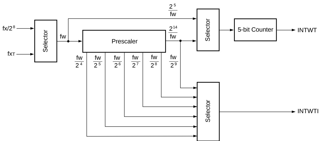
Figure 5-9: Watch Timer Block Diagram
