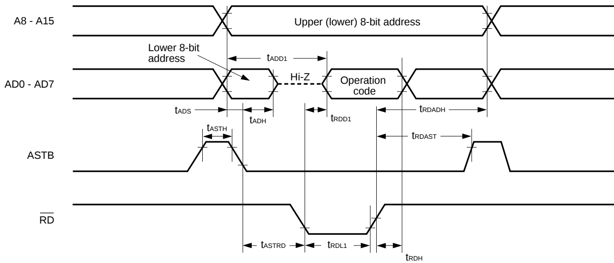
Figure 12-5: External fetch (no wait)
