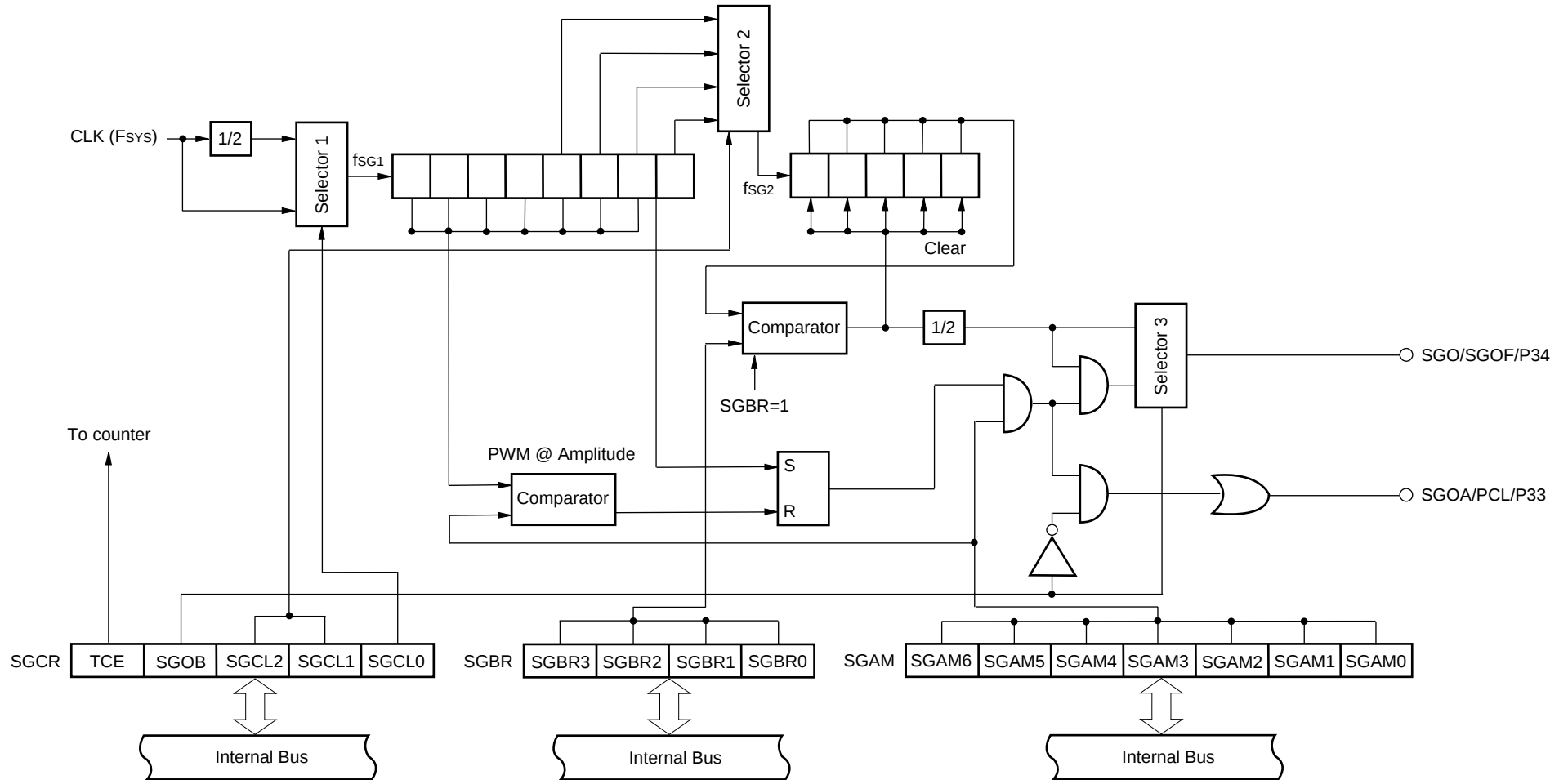
Figure 5-12: Block Diagram of the Sound Generator
