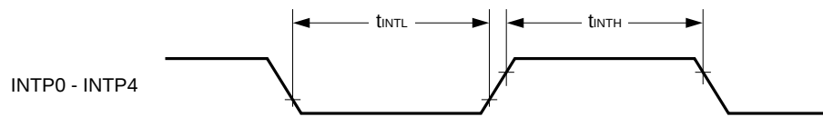
Figure 12-13: Interrupt Input Timing
