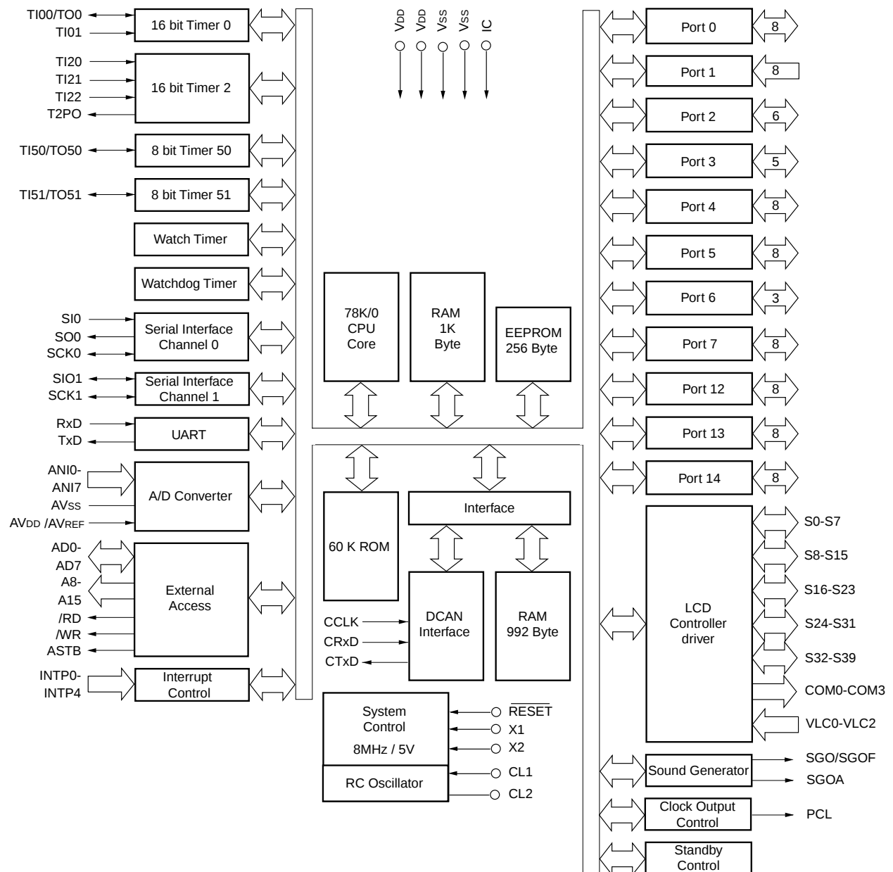
Figure 2-1: Block Diagram
