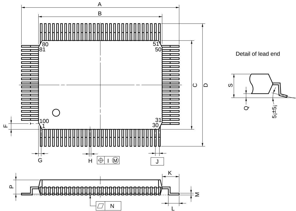
Figure 13-1: Package Drawing
