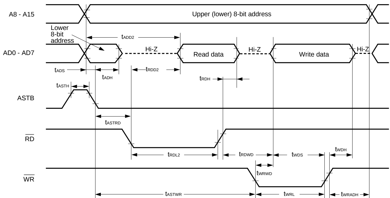
Figure 12-8: External data access (wait insertion)
