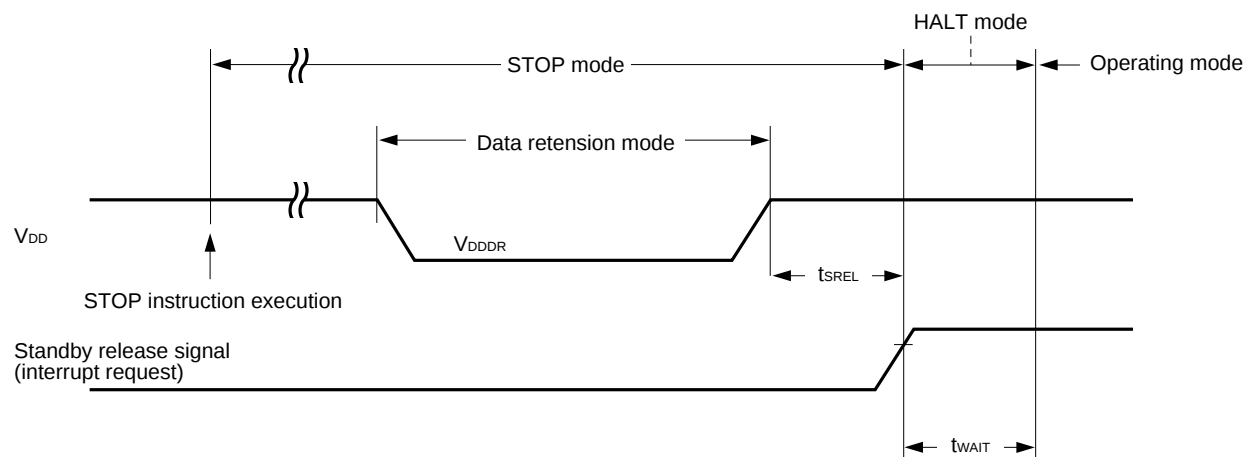
Figure 12-12: Data Retention Timing (Standby release signal: STOP mode release by interrupt signal)
