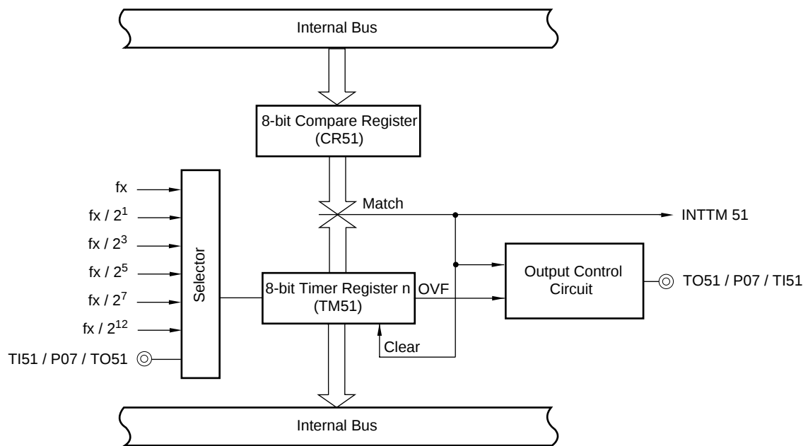
Figure 5-7: 8-Bit Timer/Event Counter 51 Block Diagram
