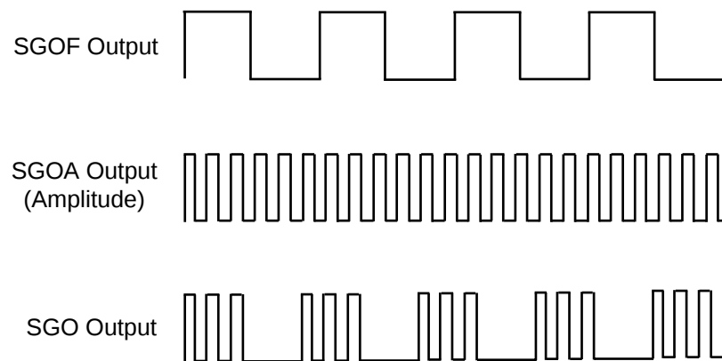
Figure 5-13: Composed Sound Generator Output SGO
