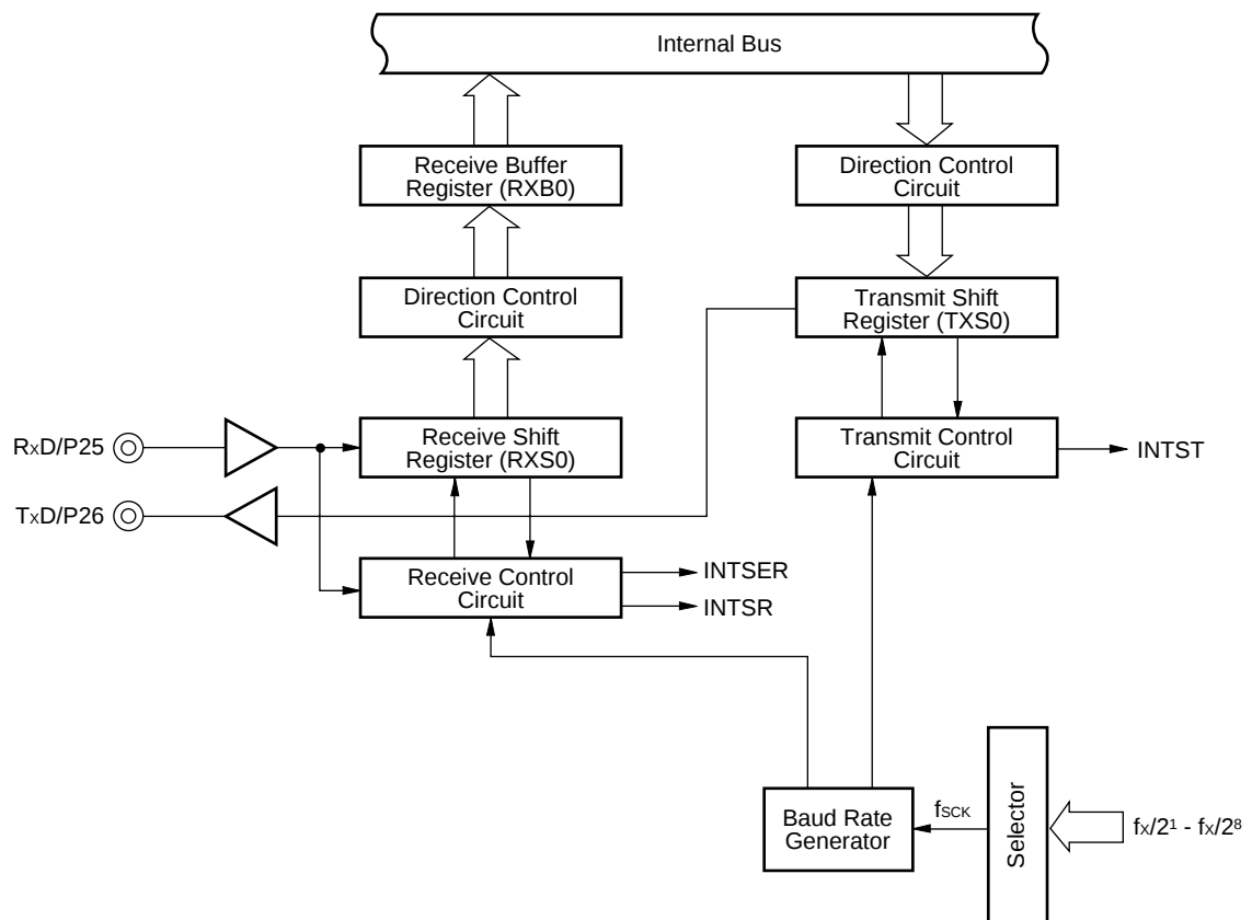
Figure 5-18: Serial Interface UART Block Diagram
