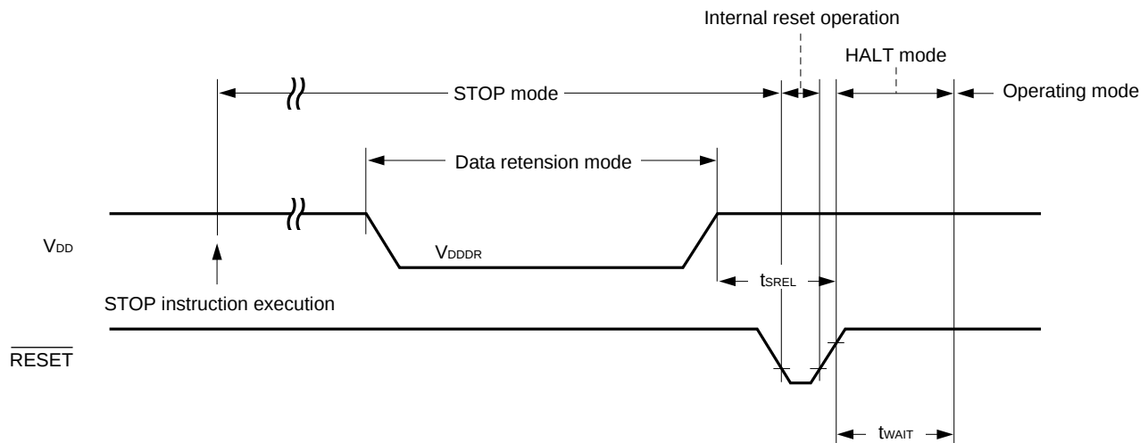
Figure 12-11: Data Retention Timing (STOP mode release by RESET)
