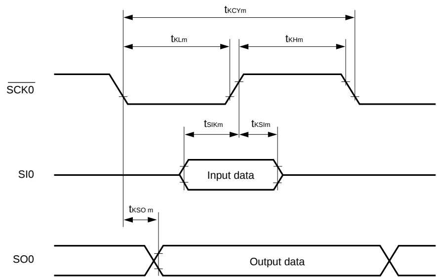
Figure 12-9: 3-wire serial I/O mode
