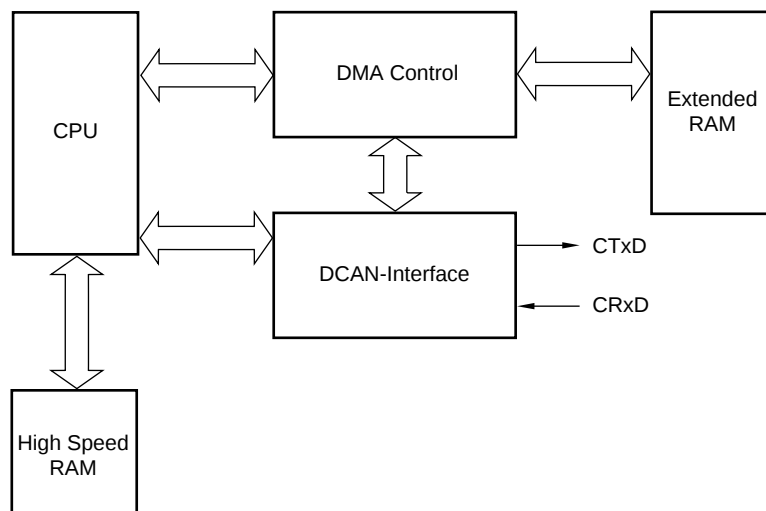
Figure 5-19: CAN-Bus Interface
