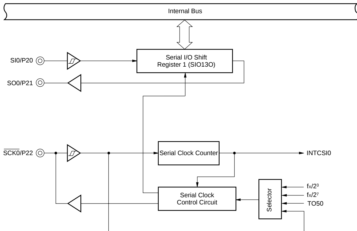
Figure 5-16: Serial Interface Channel 0 Block Diagram
