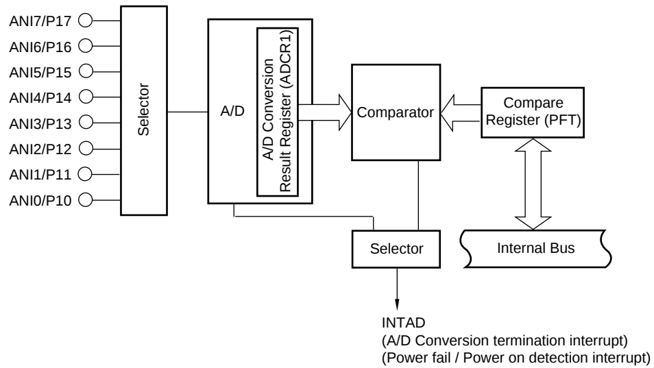
Figure 5-15: Block Diagram Power Fail Detector
