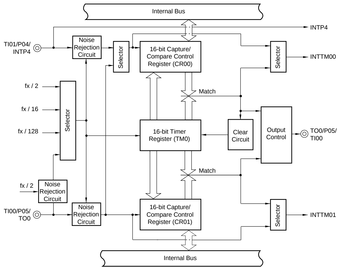
Figure 5-4: 16 bit Timer TM0
