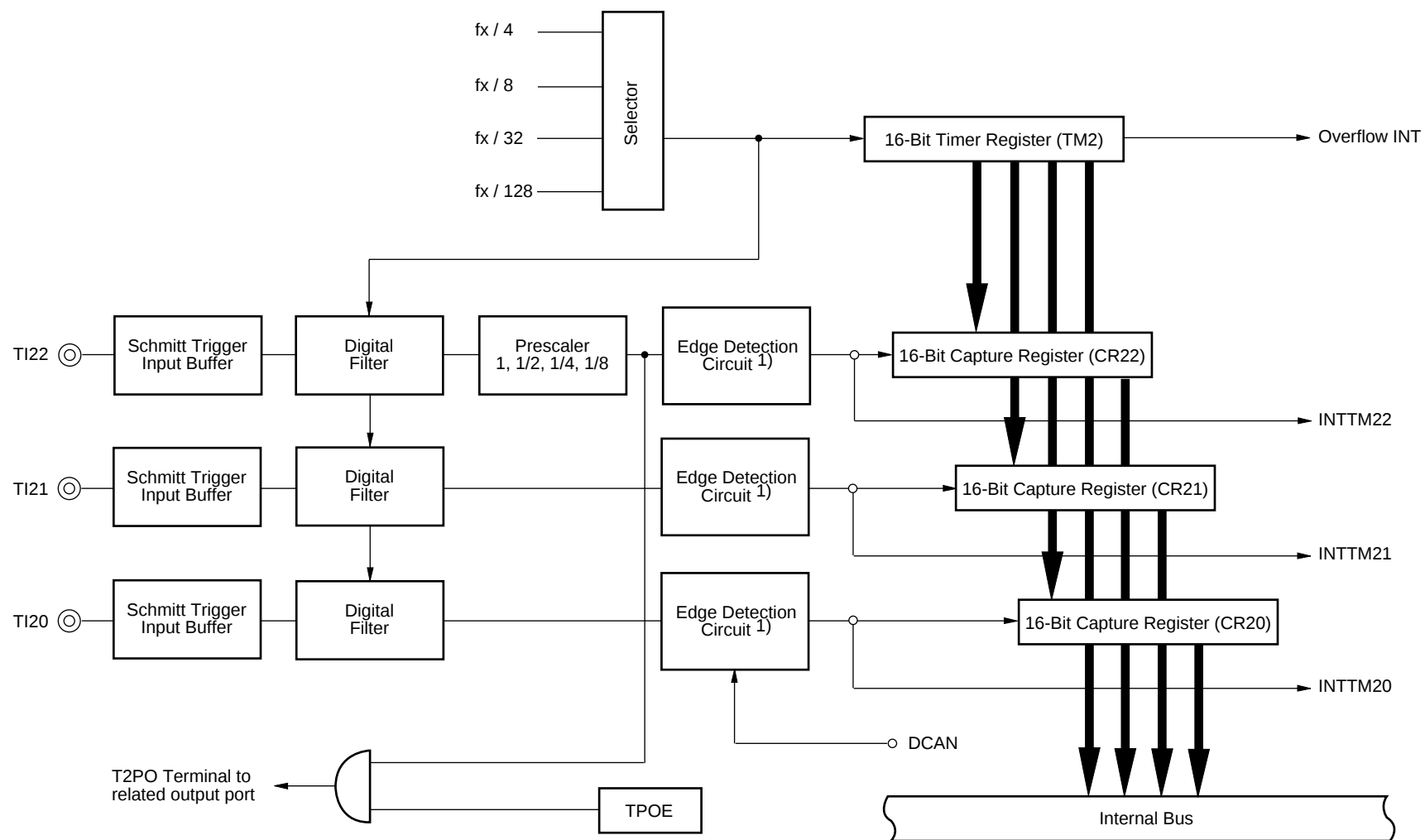
Figure 5-5: 16 Bit Timer TM2
