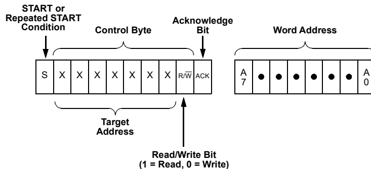
Figure 98: Basic Command Structure
