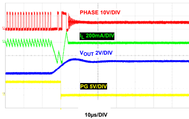
FIGURE 47. OVERVOLTAGE PROTECTION
