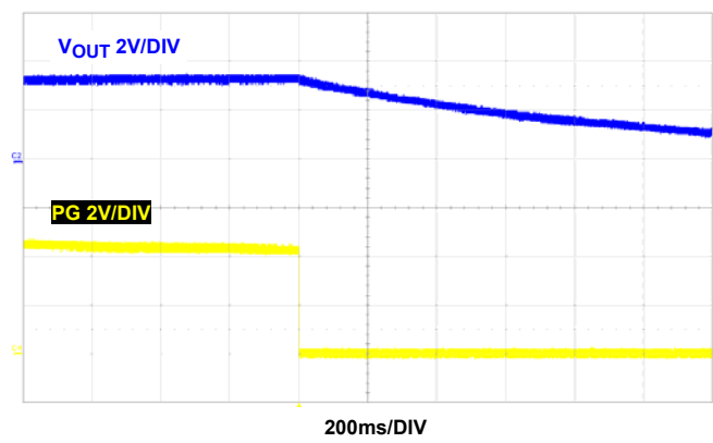
FIGURE 48. OVERTEMPERATURE PROTECTION
