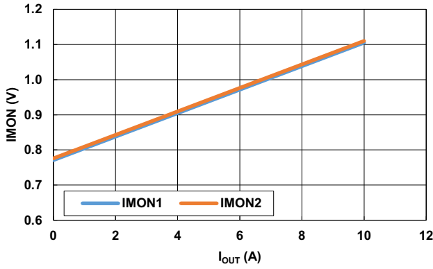
Figure 18. Output Current I_{OUT} (DC) vs IMON Pin Voltage, R_{S\_OUT} = 4m\Omega , R_{IMON} = 40.2k
