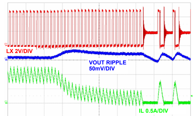
FIGURE 18. MODE TRANSITION CCM TO DCM, (5 \mu\text{s}/\text{DIV} )
