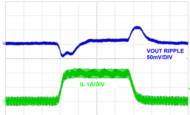
FIGURE 20. LOAD TRANSIENT (PWM), (50 \mu\text{s}/\text{DIV} )
