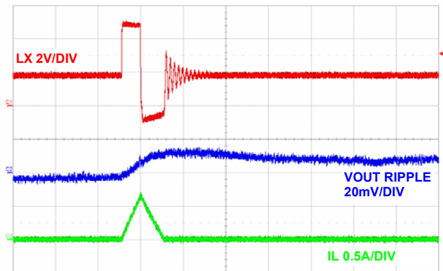
FIGURE 16. STEADY STATE OPERATION AT NO LOAD (PFM), (1 \mu\text{s}/\text{DIV} )
